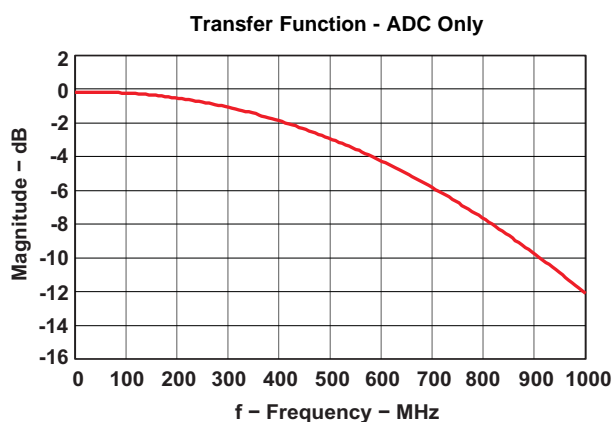
Figure 42. Analog Input Bandwidth (Data From Actual Silicon)
