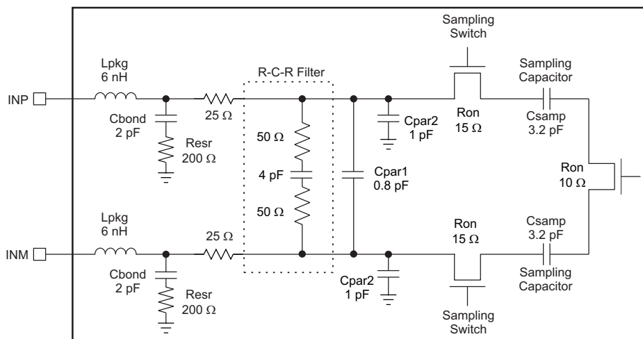
Figure 41. Input Stage
