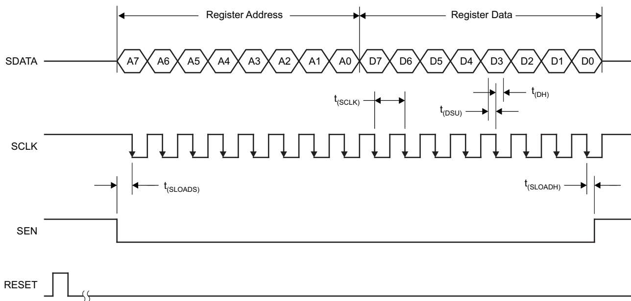
Figure 5. Serial Interface Timing Diagram
