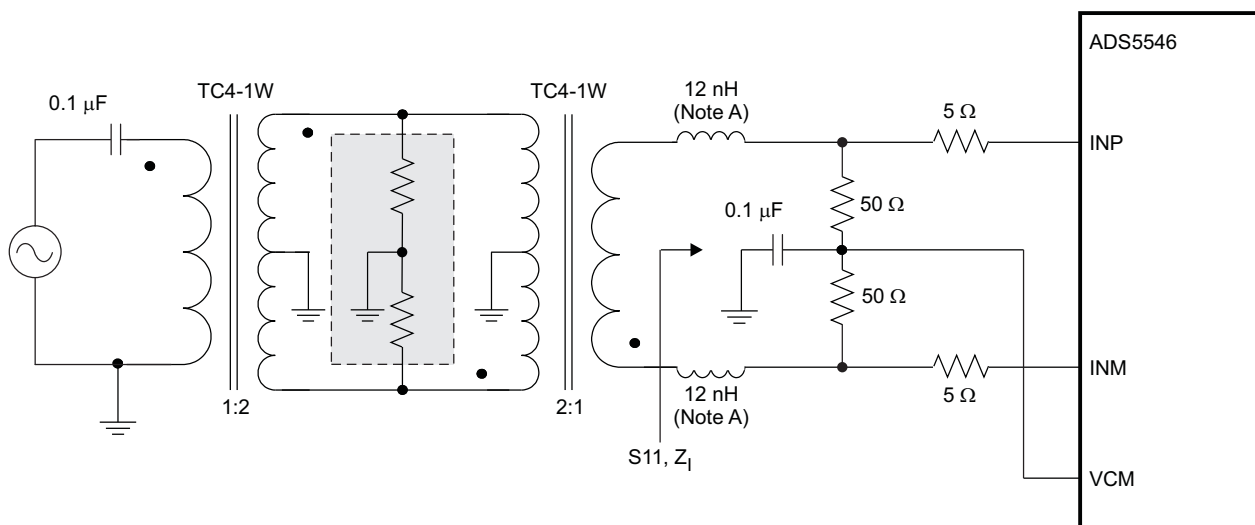
Figure 46. Configuration for Higher Input Frequencies
