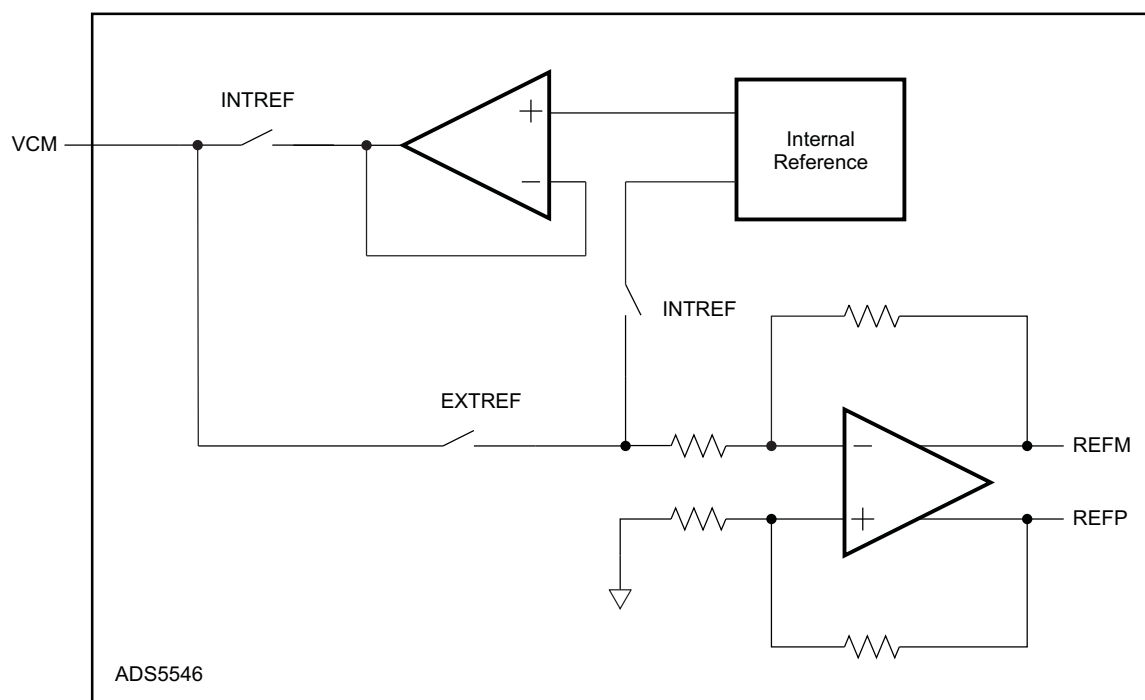
Figure 49. Reference Section
