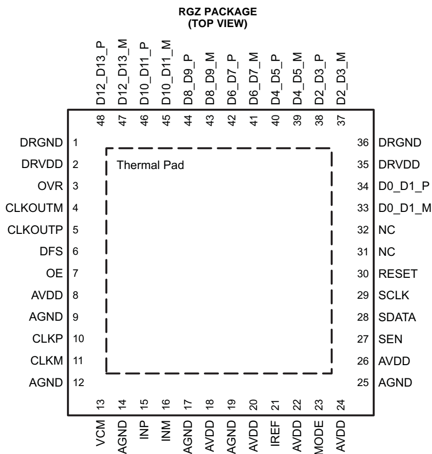
Figure 7. LVDS Mode Pinout
