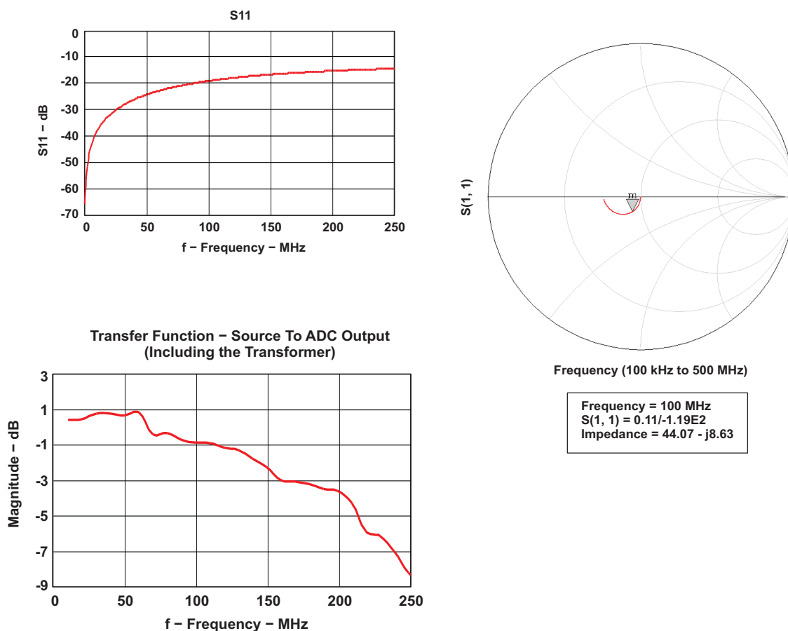
Figure 45. S11, Input Impedance and Transfer Function for the Configuration in Figure 44
