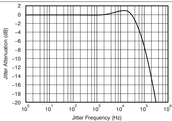
Figure 4. DIR Jitter Attenuation Characteristics
