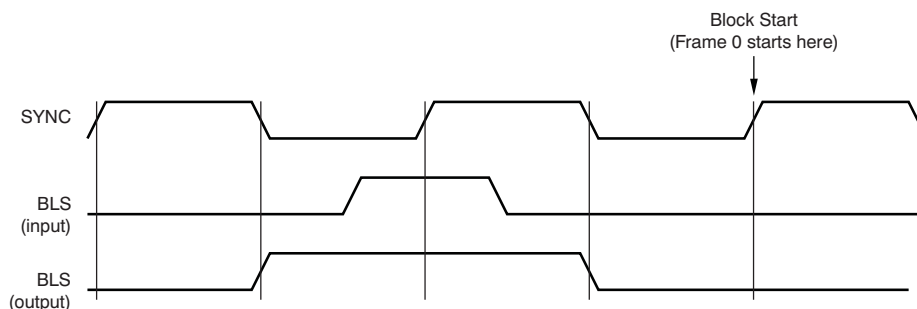
Figure 12. DIT Block Start Timing
