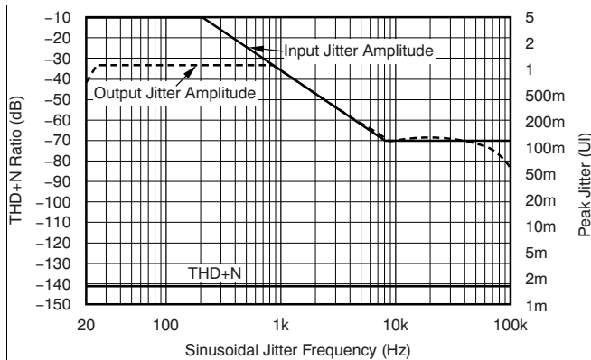
Figure 5. DIR Jitter Tolerance Plot
