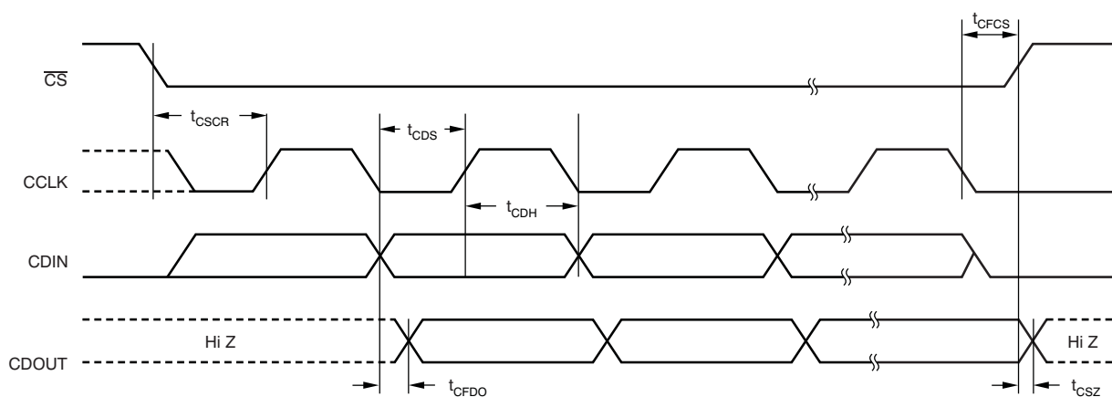
Figure 2. SPI Timing
