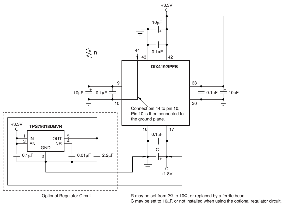
Figure 71. Recommended Power-Supply Connections
