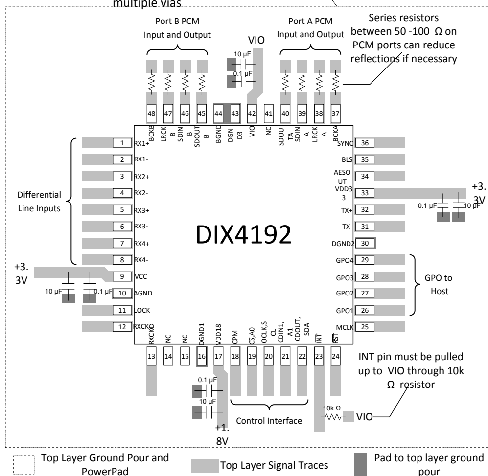
Figure 85. DIX4192 Board Layout
