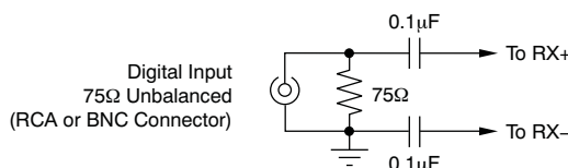
(b) Unbalanced Line Interface Without Transformer
