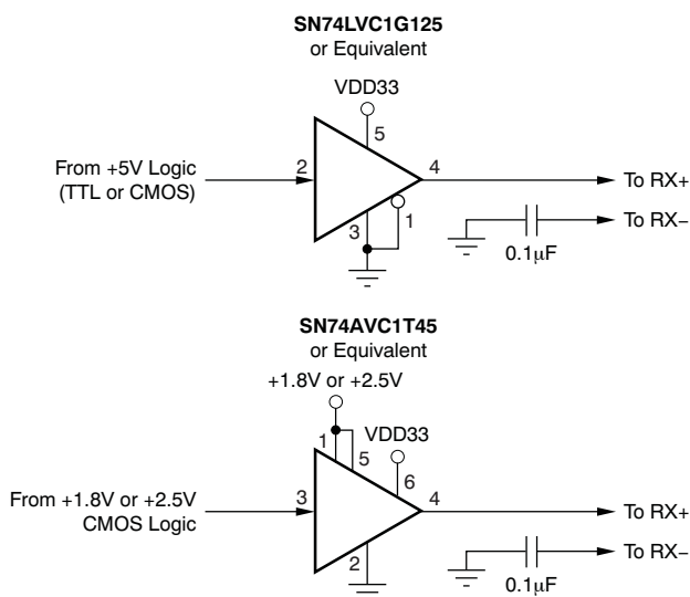
Figure 76. CMOS and TTL Input Logic Interface
