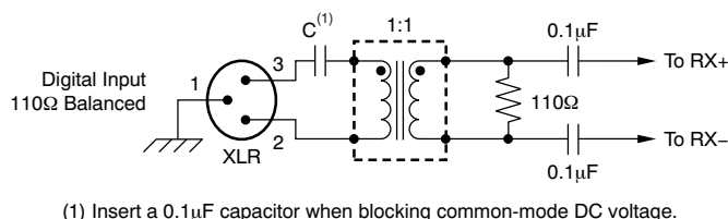
Figure 72. Transformer-Coupled Balanced Input Interface
