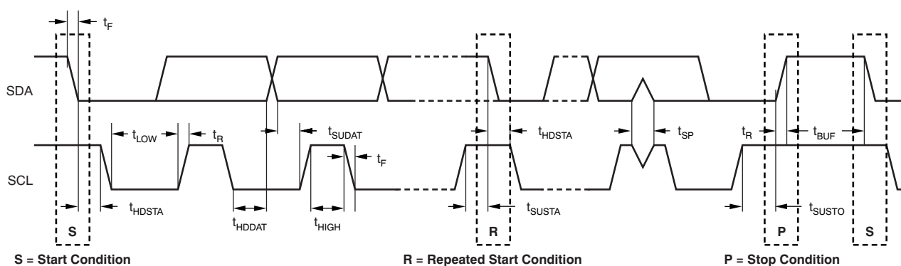
Figure 3. I 2 C Standard and Fast Mode Timing
