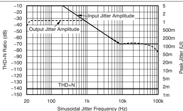
Figure 16. DIR Jitter Tolerance Plot
