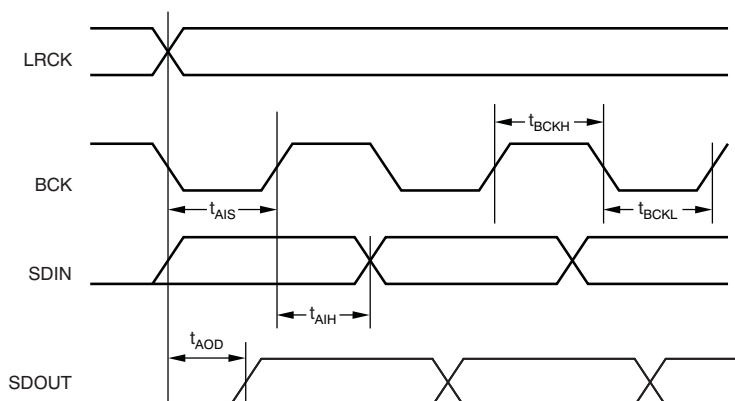
Figure 1. Audio Serial Port Timing
