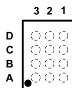
YZT Package 12-Pin DSBGA Top View
