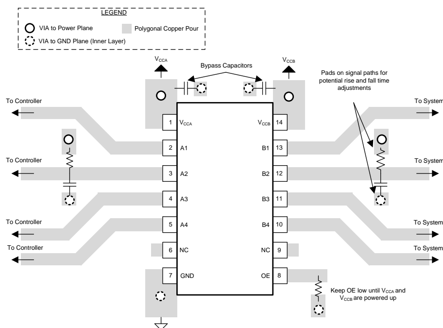
Figure 13. TXS0104E Layout Example
