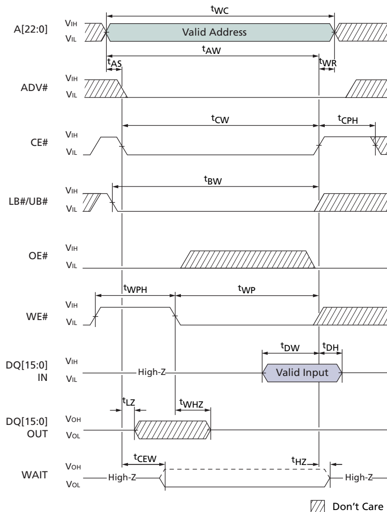
Figure 39: CE#-Controlled Asynchronous WRITE
