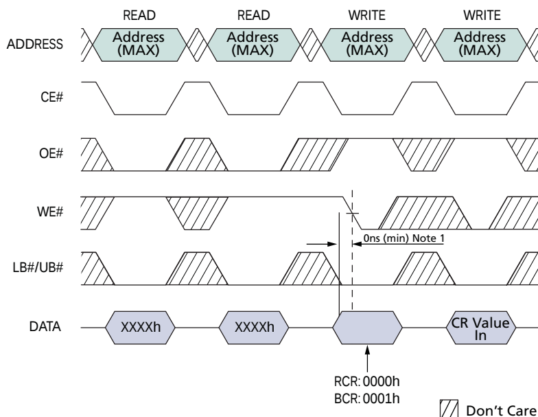
Figure 16: Load Configuration Register
