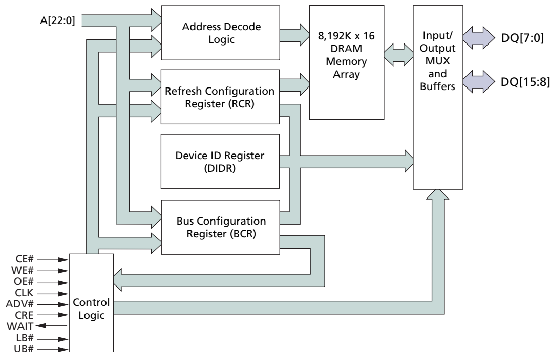
Figure 2: Functional Block Diagram – 8 Meg x 16
