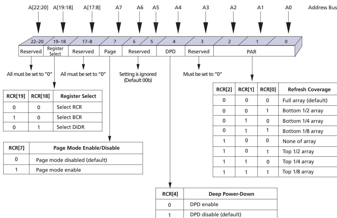
Figure 24: Refresh Configuration Register Mapping
