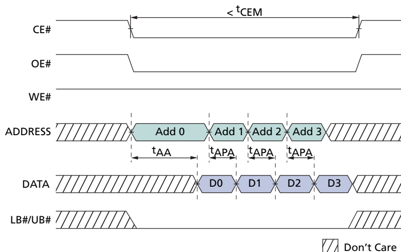
Figure 7: Page Mode READ Operation (ADV# LOW)
