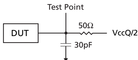
Figure 27: AC Output Load Circuit
