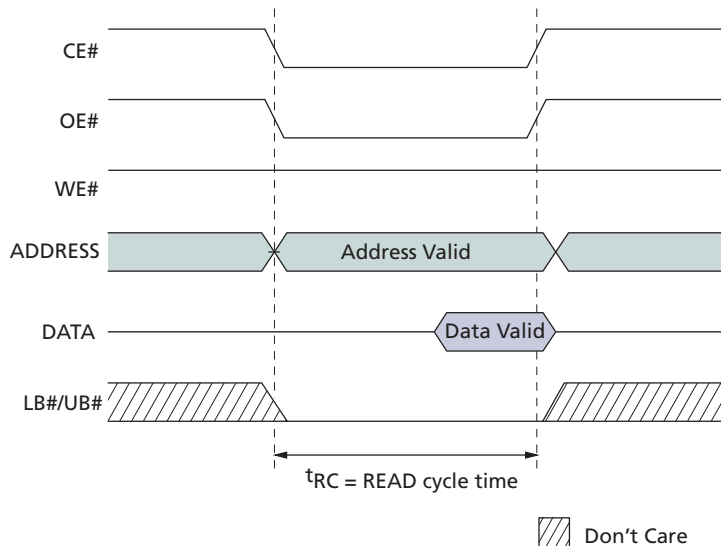
Figure 5: READ Operation (ADV# LOW)
