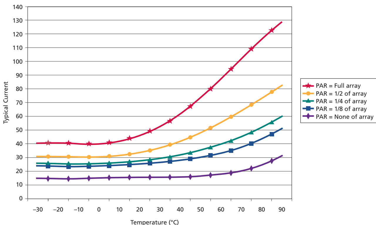
Figure 25: Typical Refresh Current vs. Temperature (ItCR)
