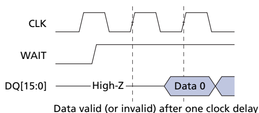
Figure 20: WAIT Configuration (BCR[8] = 1)
