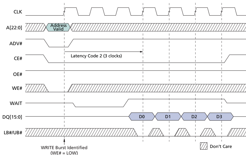
Figure 9: Burst Mode WRITE (4-word burst)
