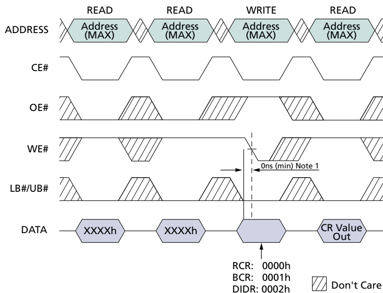
Figure 17: Read Configuration Register
