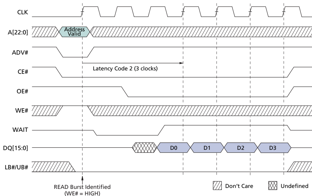
Figure 8: Burst Mode READ (4-word burst)
