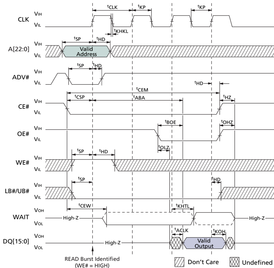
Figure 33: Single-Access Burst READ Operation – Variable Latency
