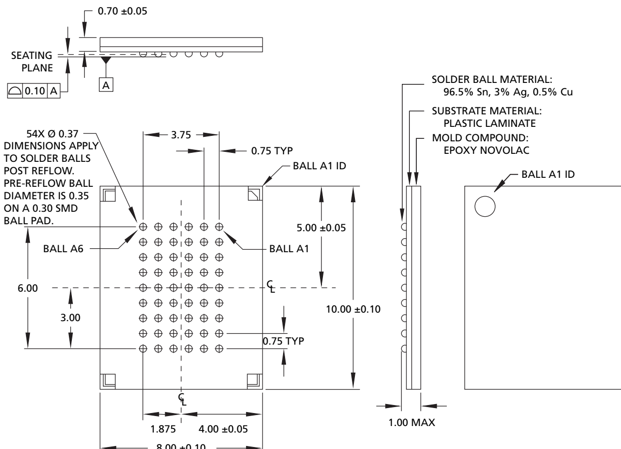
Figure 56: 54-Ball VFBGA
