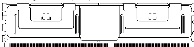
Figure 1: 240-Pin FBDIMM (MO-256 R/C B)
