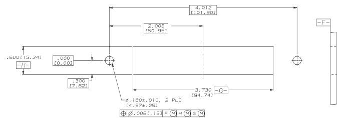
PANEL DIMENSIONS
