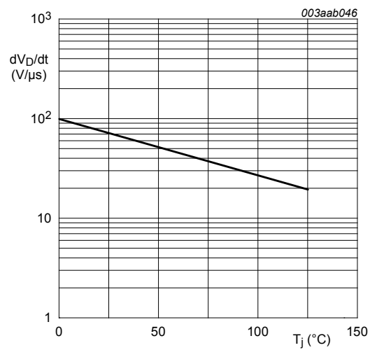
Fig. 12. Rate of rise of off-state voltage as a function of junction temperature; typical values
