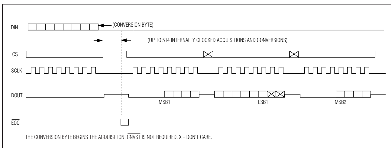
Figure 6. Clock Mode 10
