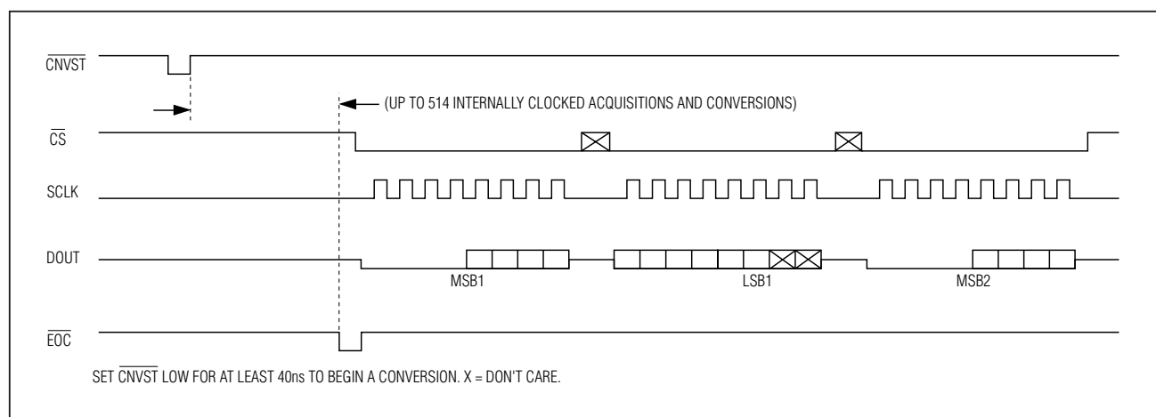
Figure 4. Clock Mode 00
