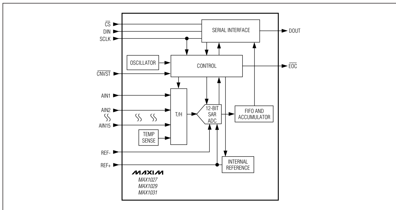
Figure 2. Functional Diagram
