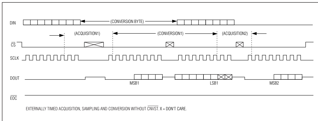
Figure 7. Clock Mode 11
