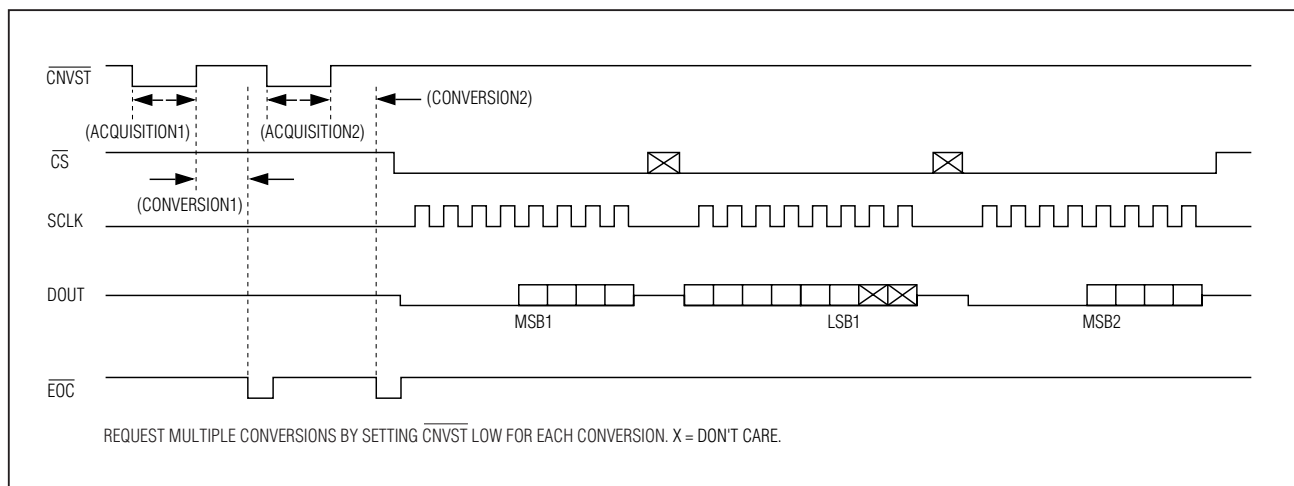
Figure 5. Clock Mode 01
