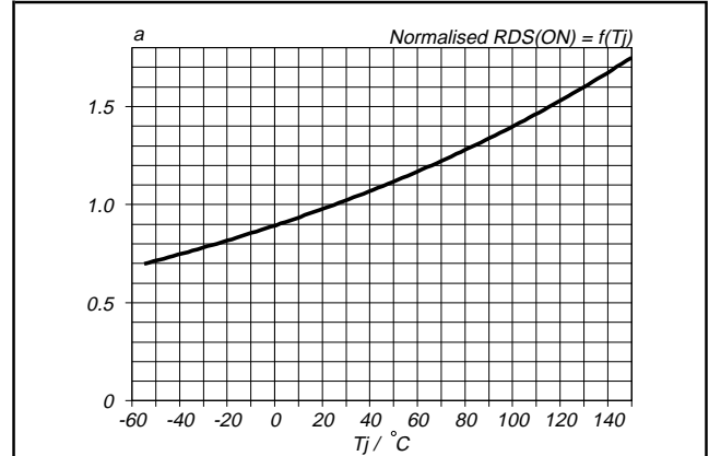
Fig.13. Normalised drain-source on-state resistance. a = R_{DS(ON)}/R_{DS(ON)25^\circ\text{C}} = f(T_j) ; I_D = 25\ \text{A} ; V_{IS} \geq 5\ \text{V}
