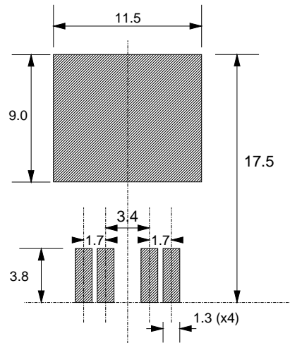
soldering pattern for surface mounting.
