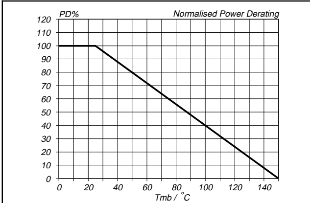
Fig. 4. Normalised limiting power dissipation. P_D\% = 100 \cdot P_D / P_D(25^\circ\text{C}) = f(T_{mb})
