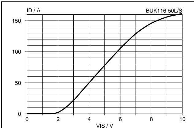
Fig.11. Typical transfer characteristics, T_j = 25^\circ\text{C} . I_D = f(V_{IS}) ; conditions: V_{DS} = 12\ \text{V} ; t_p = 250\ \mu\text{s}
