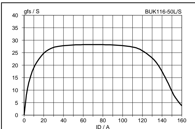
Fig.12. Typical transconductance, T_j = 25^\circ\text{C} . g_{fs} = f(I_D) ; conditions: V_{DS} = 12\ \text{V} ; t_p = 250\ \mu\text{s}
