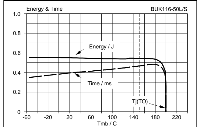
Fig.19. Typical overload protection characteristics. Conditions: V_{DD} = 13 V ; V_{PS} = V_{PSN} ; V_{IS} = 8 V ; SC load
