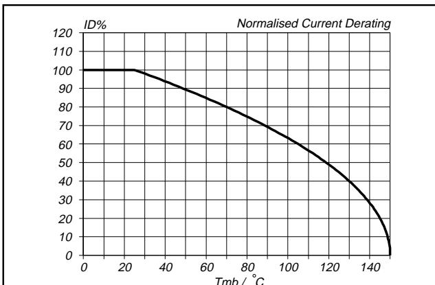
Fig. 5. Normalised continuous drain current. I_D\% = 100 \cdot I_D / I_D(25^\circ\text{C}) = f(T_{mb}) ; conditions: V_{IS} = 5\text{ V}
