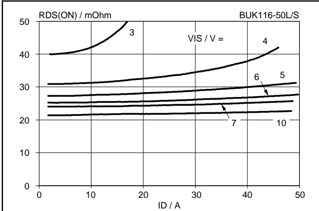
Fig.10. Typical on-state resistance, T_j = 25^\circ\text{C} . R_{DS(ON)} = f(I_D) ; parameter V_{IS} ; t_p = 250\ \mu\text{s}
