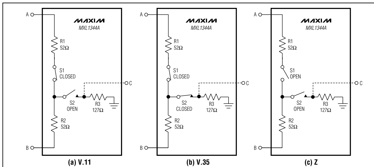
Figure 4. Termination Modes
