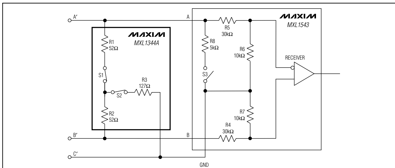
Figure 9. V.35 Termination and Internal Resistance Networks
