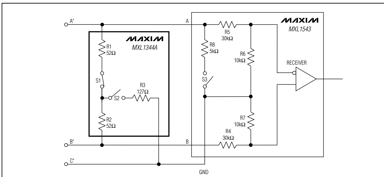
Figure 7. V.11 Termination and Internal Resistance Networks
