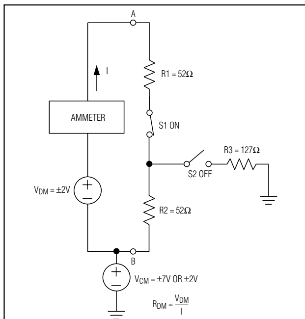
Figure 1. V.11 or V.35 Differential Impedance Measurement
