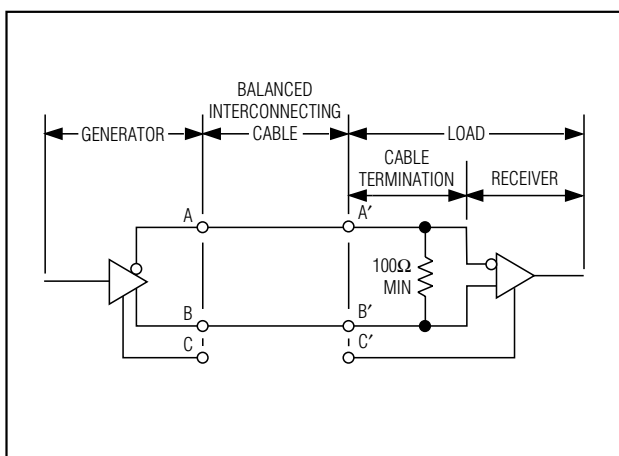
Figure 6. Typical V.11 Interface
