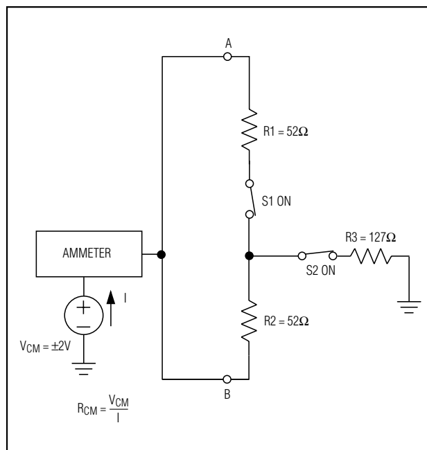
Figure 2. V.35 Common-Mode Impedance Measurement
