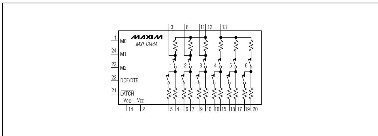
Figure 3. Block Diagram
