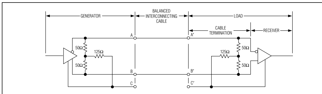
Figure 8. Typical V.35 Interface
