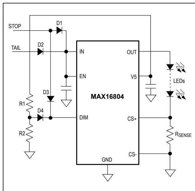
Figure 2. Two-Level Brightness Operation
