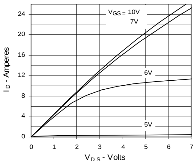
Fig. 1. Output Characteristics
