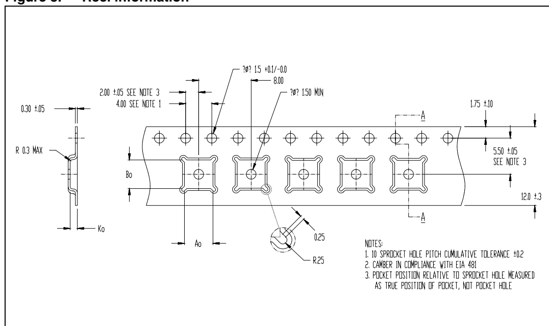
Figure 8. Reel information
