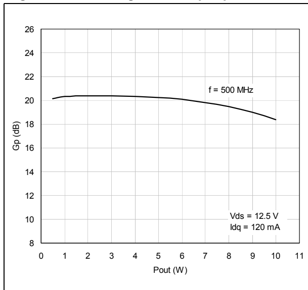
Figure 3. Power gain vs output power
