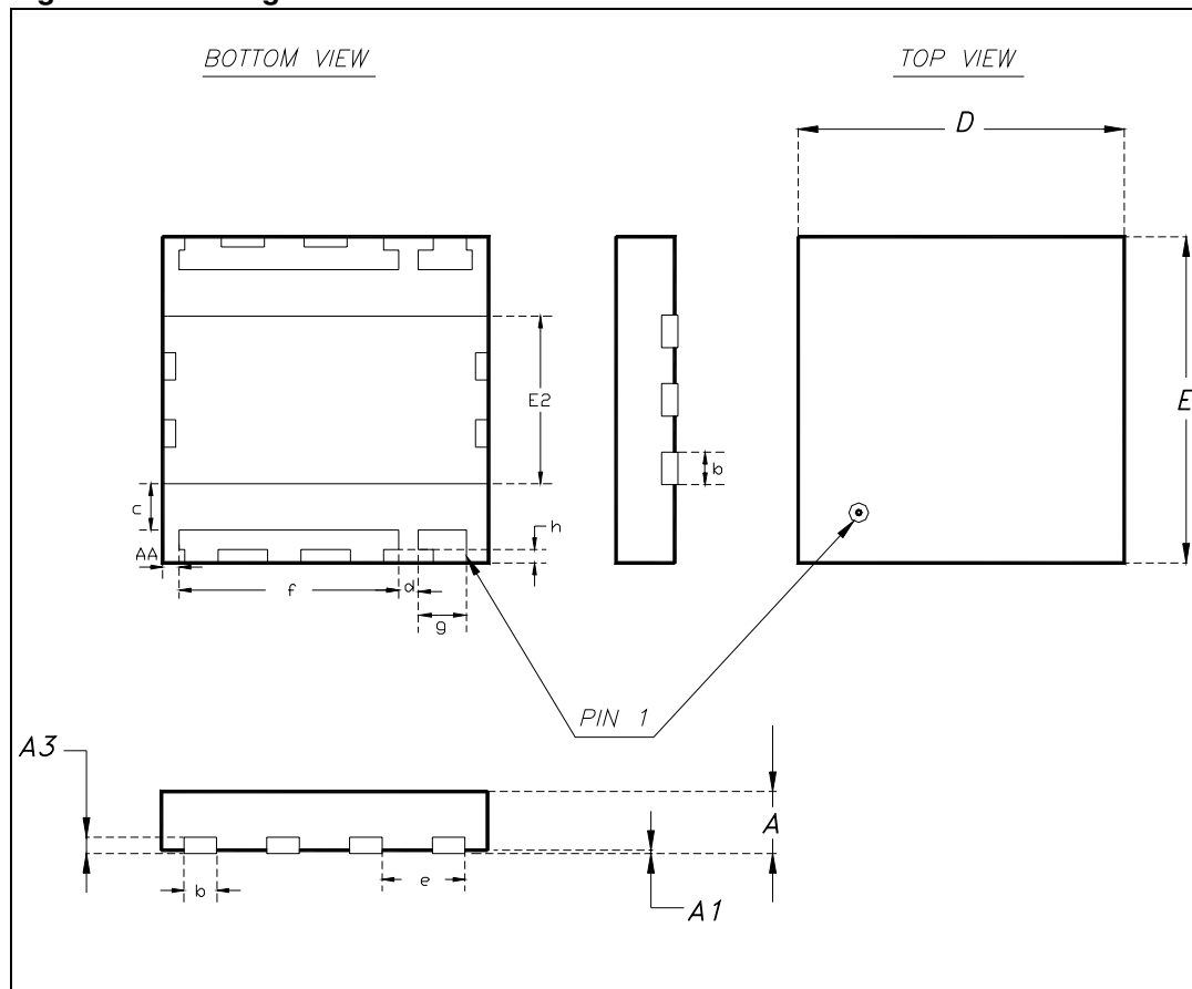
Figure 6. Package dimensions
