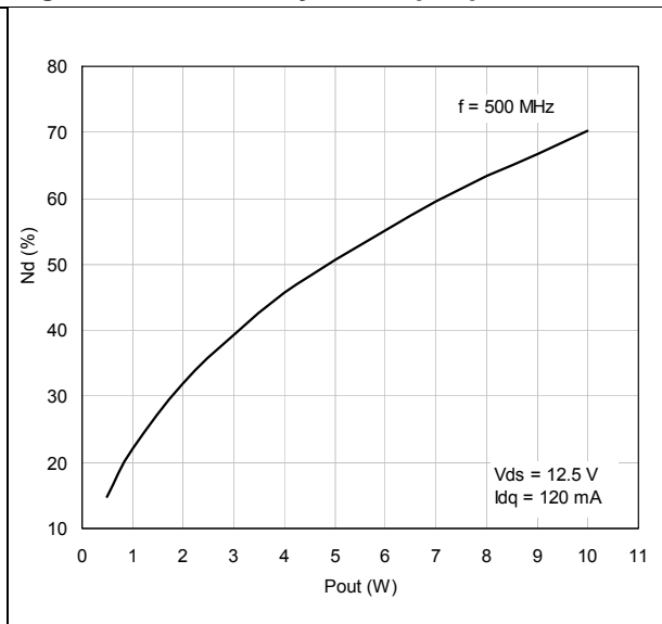
Figure 4. Efficiency vs. output power
