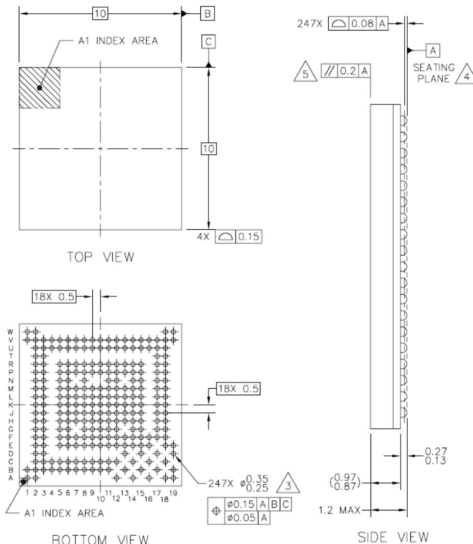
Figure 13. Package Drawing
