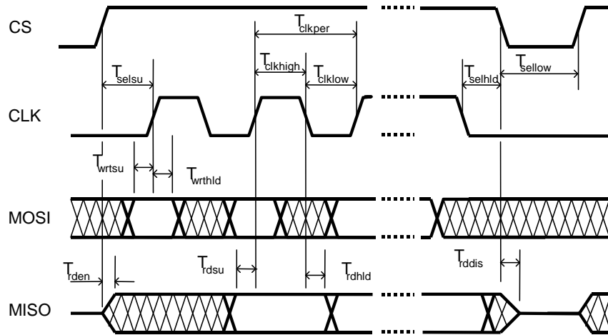
Figure 4. SPI Interface Timing Diagram
