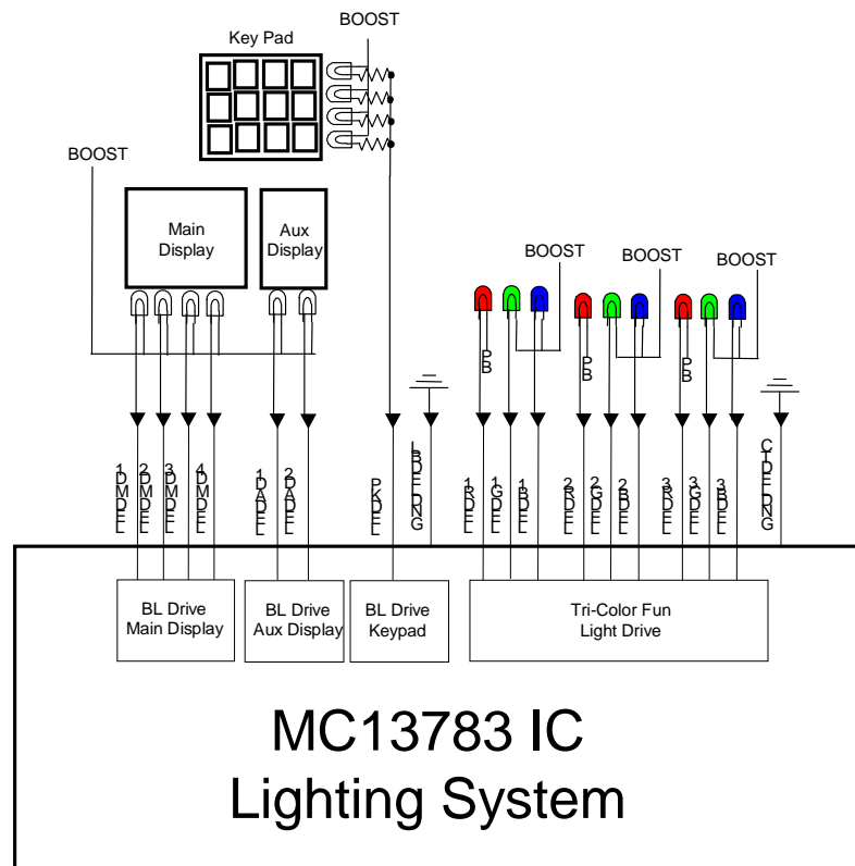
Figure 12. MC13783 Lighting System
