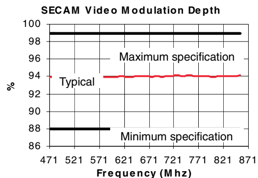
Figure 4. Typical Performance—Video
