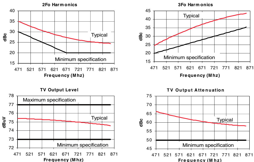
Figure 3. Typical Performance—Modulator High Frequency
