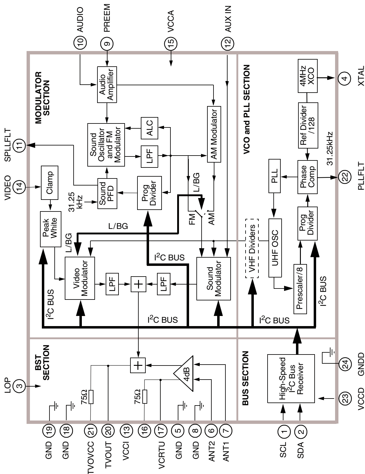
Figure 2. Simplified Block Diagram—MC44BC373/374
