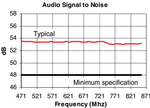
Figure 5. Typical performance—Audio
