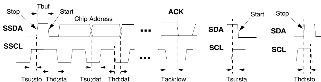
Figure 11. SSDA/SSCL Timing
