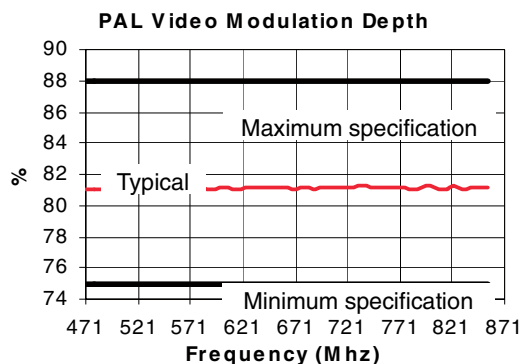
Figure 4. Typical Performance—Video
