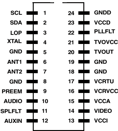
Figure 1. MC44BC373/374 Pin Connections
