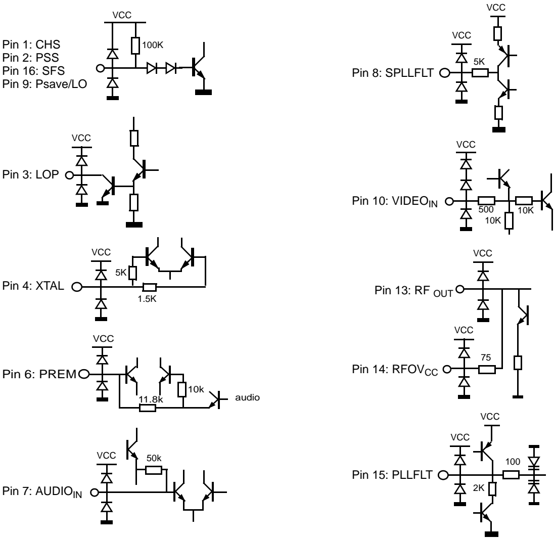
Figure 3. Pin Schematics
