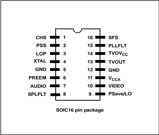
Figure 1. Pin Connections
