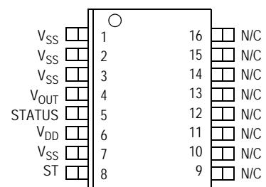
Figure 2. Pin Connections
