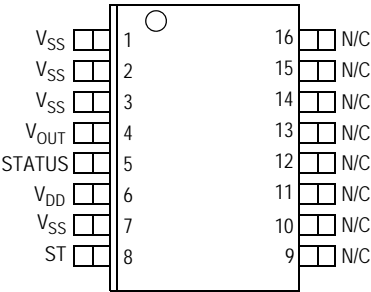
16-Pin SOIC Package N/C pins are recommended to be left FLOATING
