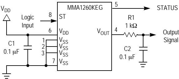
Figure 5. SOIC Accelerometer with Recommended Connection Diagram
