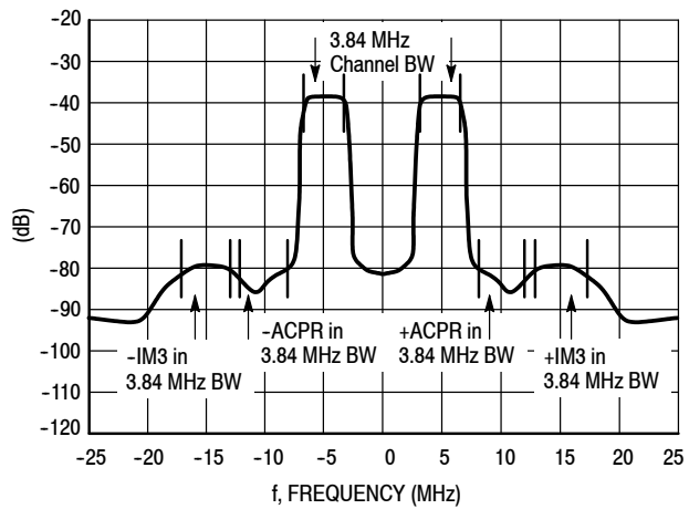
Figure 11. 2-Carrier W-CDMA Spectrum
