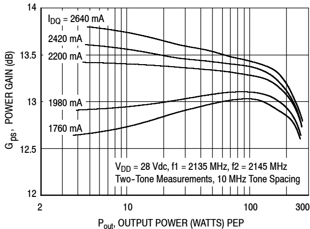
Figure 4. Two-Tone Power Gain versus Output Power
