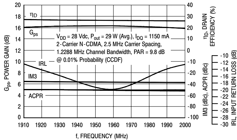
Figure 3. 2-Carrier N-CDMA Broadband Performance @ P_{out} = 29 Watts Avg.
