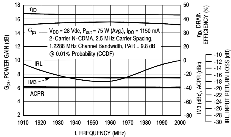
Figure 4. 2-Carrier N-CDMA Broadband Performance @ P_{out} = 75 Watts Avg.
