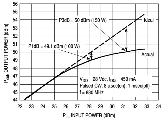
Figure 9. Pulsed CW Output Power versus Input Power
