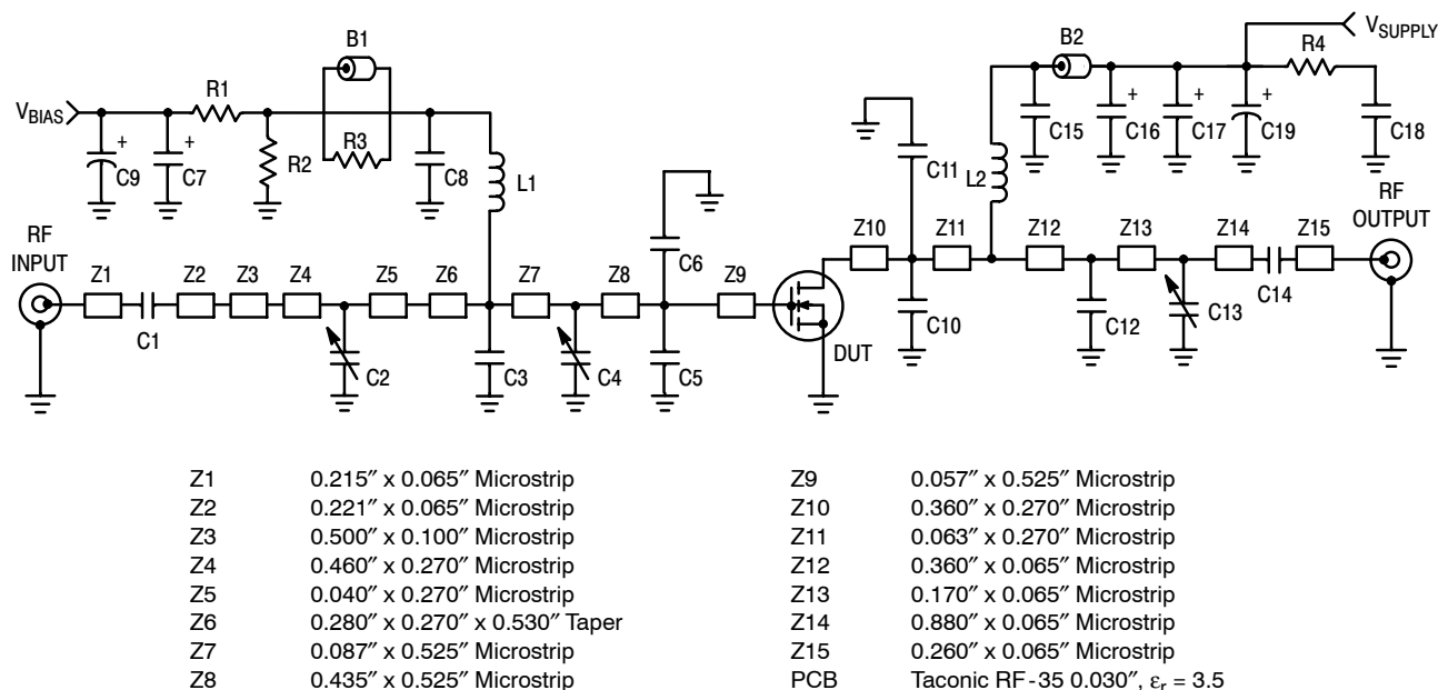
Figure 1. MRF6S9060NR1(NBR1) Test Circuit Schematic
