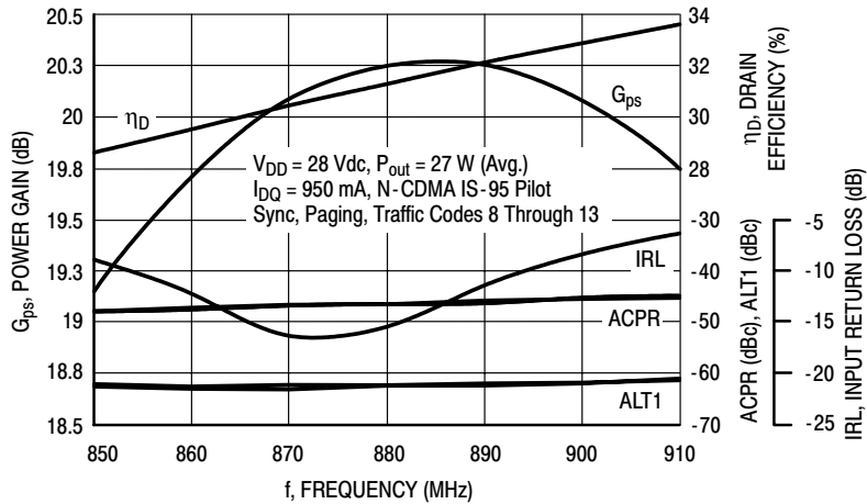
Figure 3. Single-Carrier N-CDMA Broadband Performance @ P_{out} = 27 Watts Avg.
