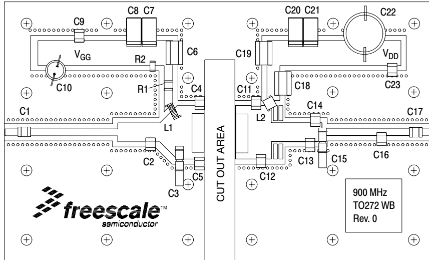
Figure 2. MRF6S9125MR1 (MBR1) Test Circuit Component Layout
