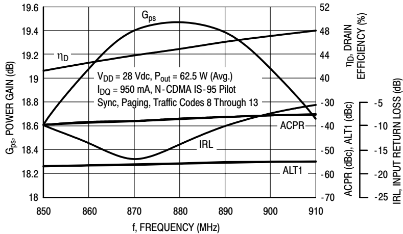
Figure 4. Single-Carrier N-CDMA Broadband Performance @ P_{out} = 62.5 Watts Avg.
