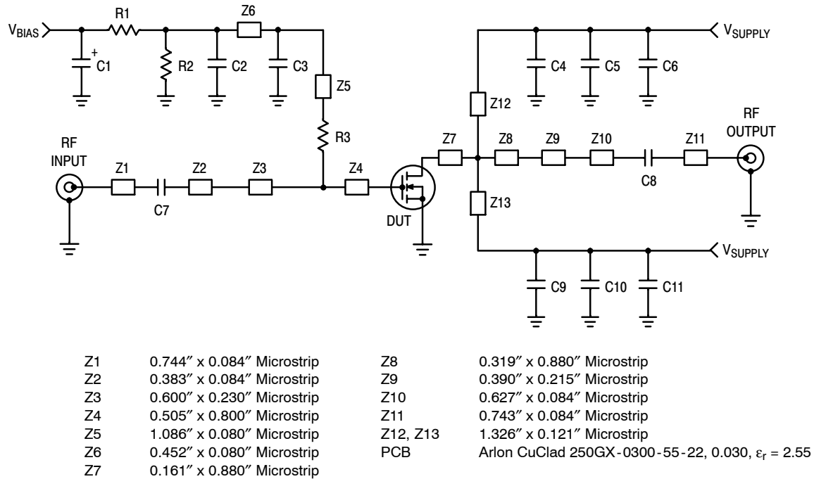
Figure 1. MRF7S19100NR1(NBR1) Test Circuit Schematic
