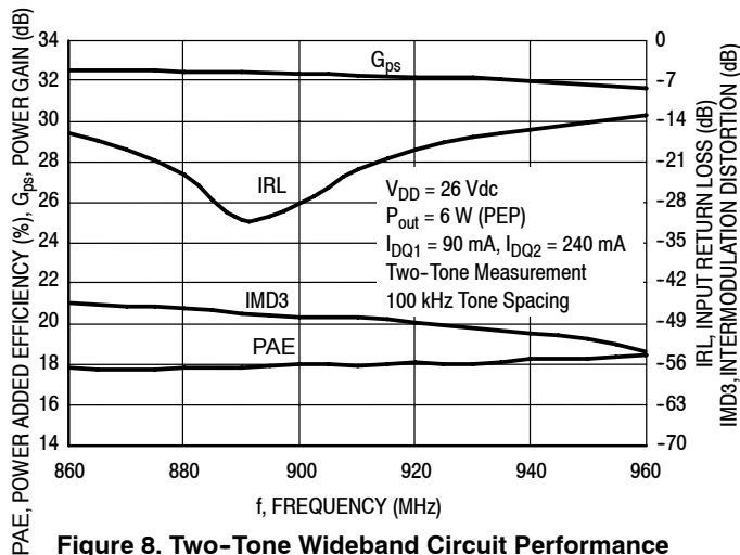
Figure 8. Two-Tone Wideband Circuit Performance @ P_{out} = 6 Watts
