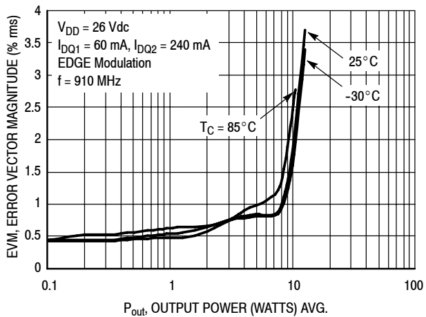
Figure 14. Error Vector Magnitude versus Output Power
