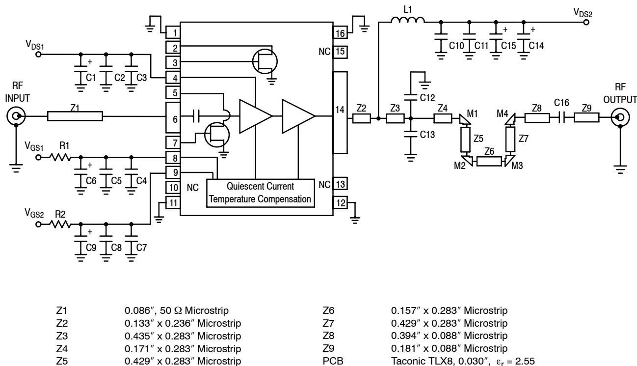
Figure 3. MW4IC915NBR1(GNBR1) Test Fixture Schematic
