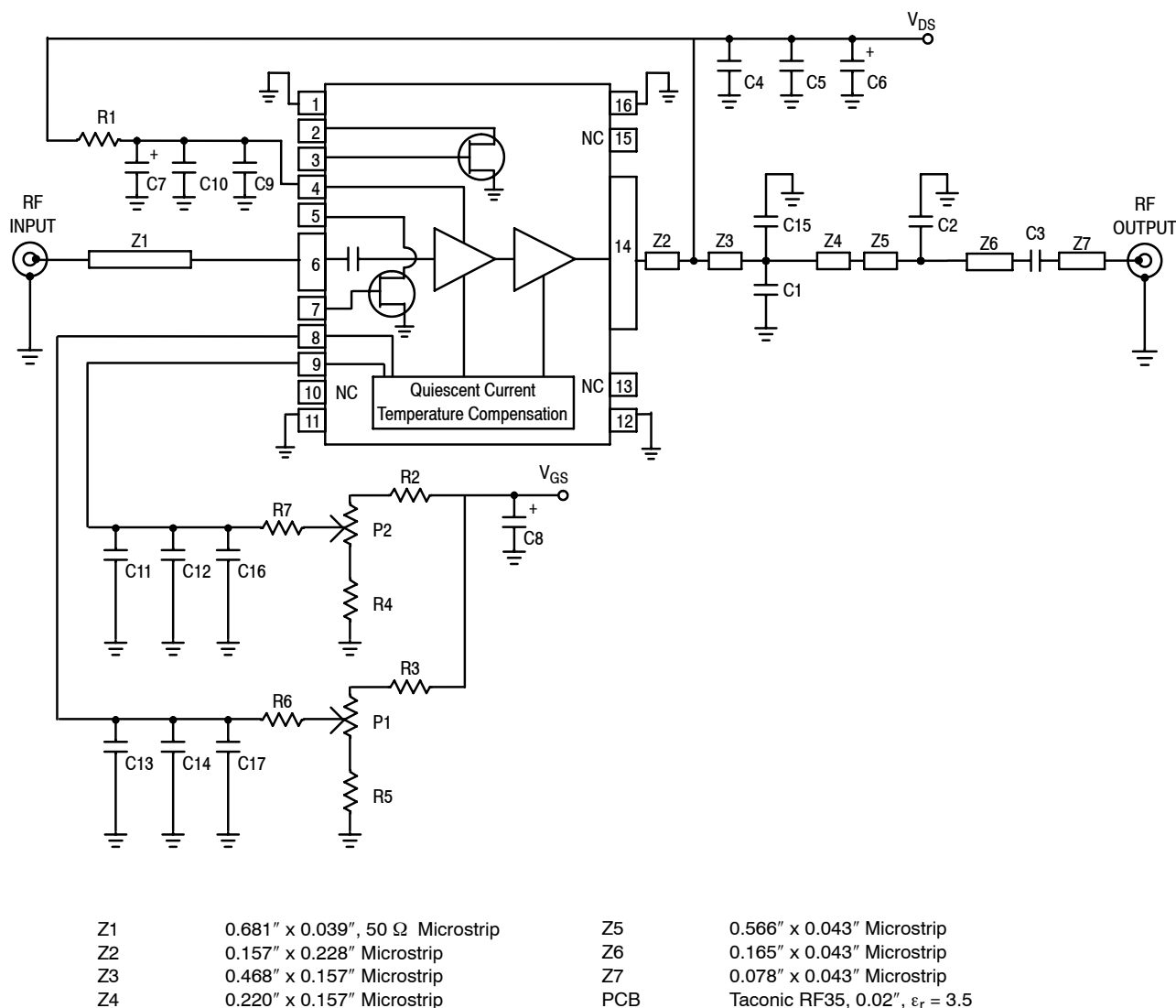
Figure 5. MW4IC915NBR1(GNBR1) Reference Board Schematic
