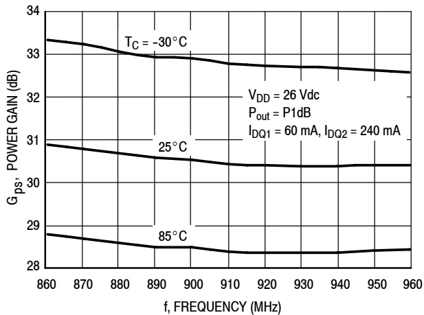
Figure 12. Power Gain versus Frequency
