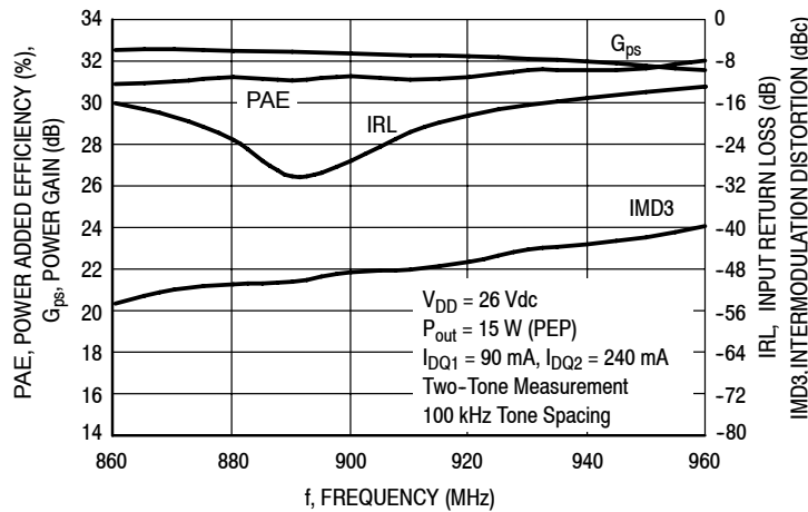
Figure 7. Two-Tone Wideband Circuit Performance @ P_{out} = 15 Watts PEP
