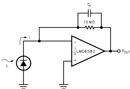
FIGURE 17. Photodiode Amplifier
