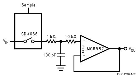
FIGURE 22. Sample-and-Hold Application
