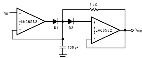
FIGURE 18. Low Voltage Peak Detector
