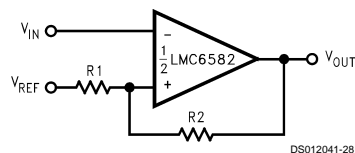
FIGURE 20. Comparator with Hysteresis
