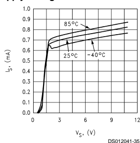
Supply Current Per Amplifier vs Supply Voltage
