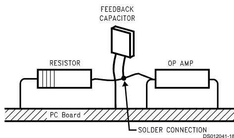
FIGURE 13. Air Wiring
