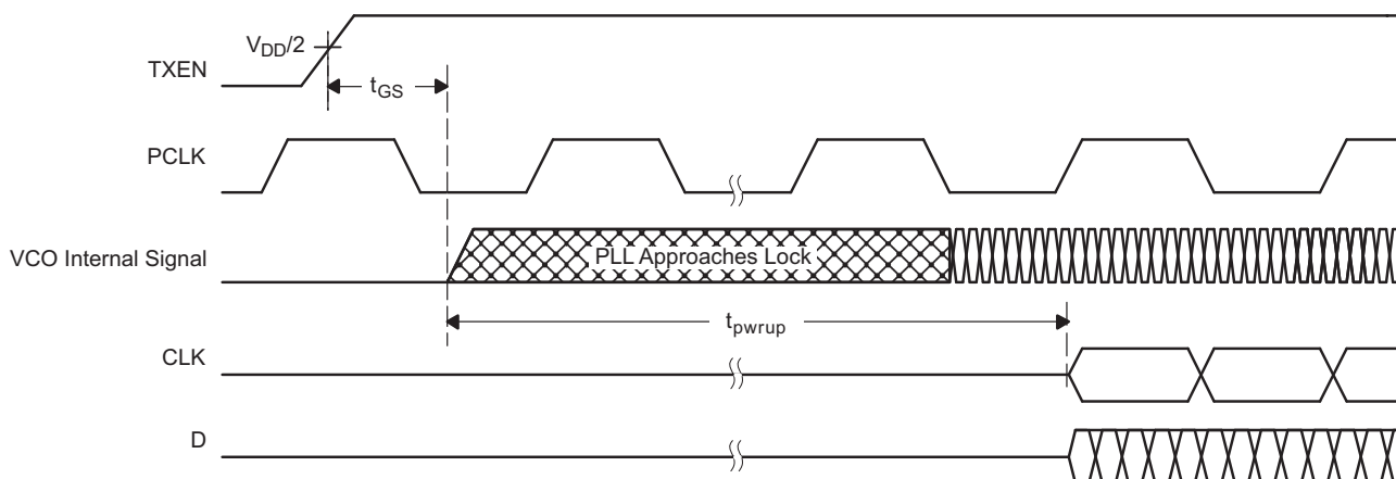
Figure 12. Transmitter Behavior While Approaching Sync
