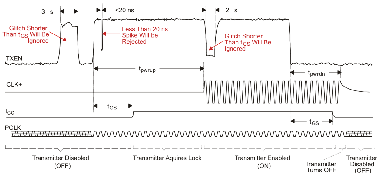
Figure 13. Transmitter Enable Glitch Suppression Time
