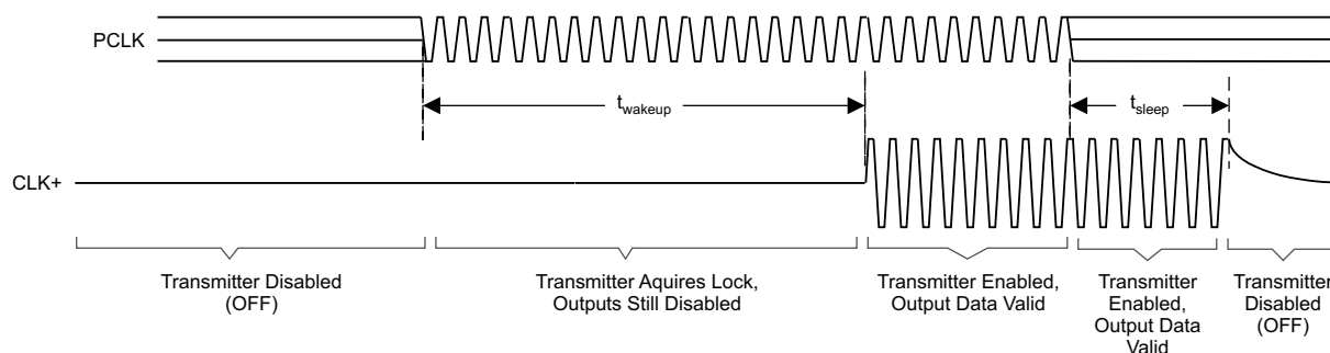
Figure 14. Standby Detection
