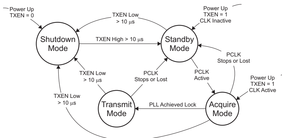
Figure 4. Status Detect and Operating Modes Flow Diagram
