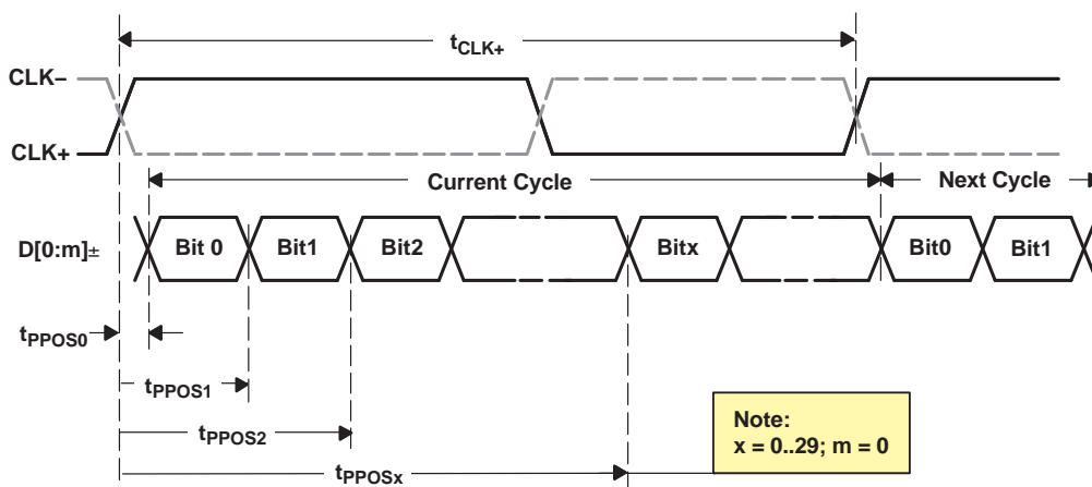
Figure 11. t_{SK(0)} SubLVDS Output Pulse Position Measurement
