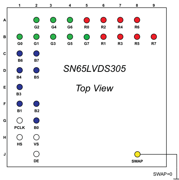
Figure 1. SWAP TERMINAL = 0
