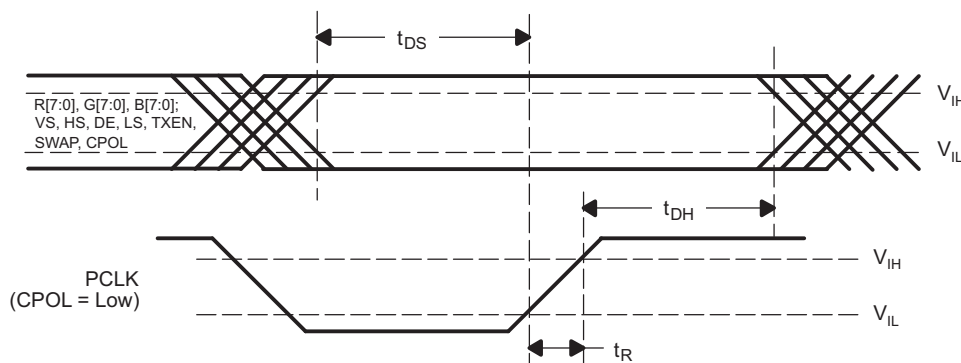
Figure 6. Setup/Hold Time
