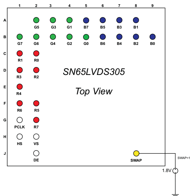
Figure 2. SWAP Terminal = 1
