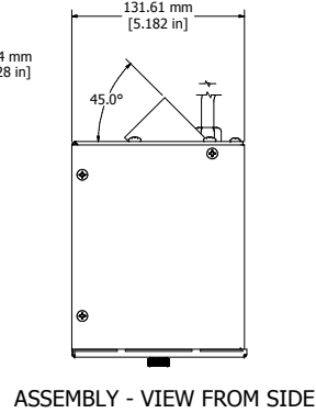
ASSEMBLY - VIEW FROM SIDE
