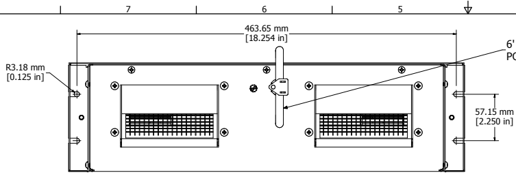
ASSEMBLY - VIEW FROM BACK
