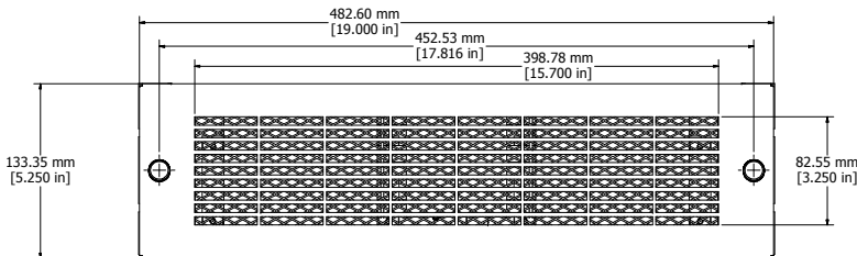
ASSEMBLY - VIEW FROM FRONT
