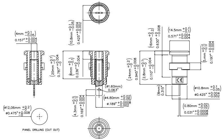
Model 72913 Panel Mount IEC61010 4mm (0.16in) Jack for Sheathed Banana Plugs
