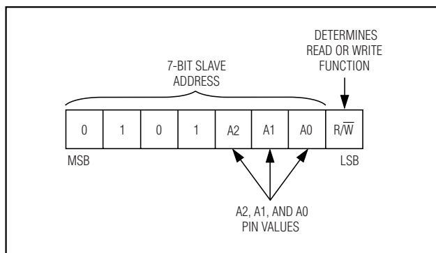
Figure 5. DS1881's Slave Address Byte
