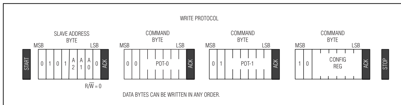
Figure 2. Write Protocol
