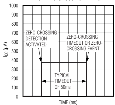
SUPPLY CURRENT vs. ZERO-CROSSING TIMING
