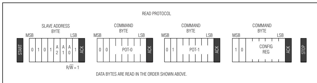
Figure 1. Read Protocol
