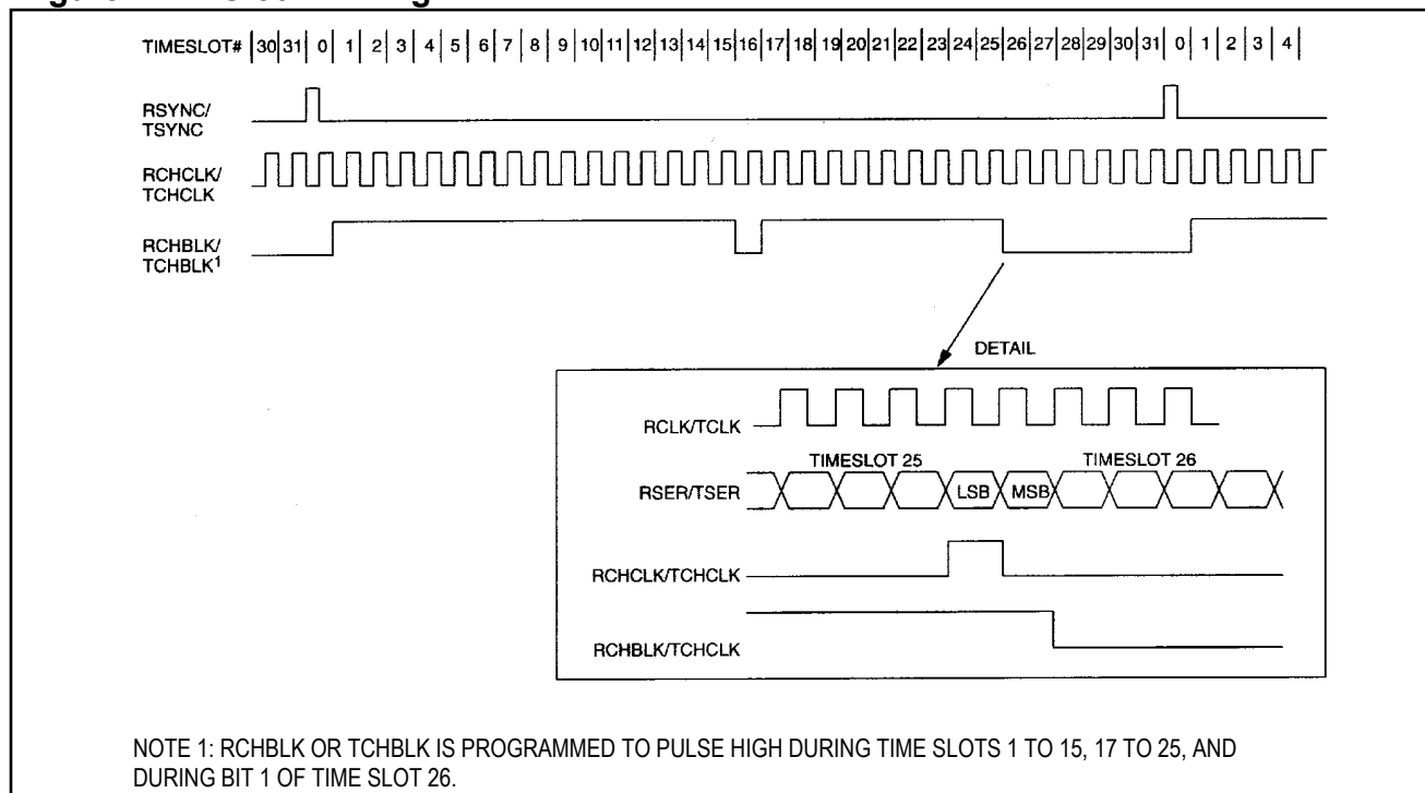
Figure 14-7. G.802 Timing
