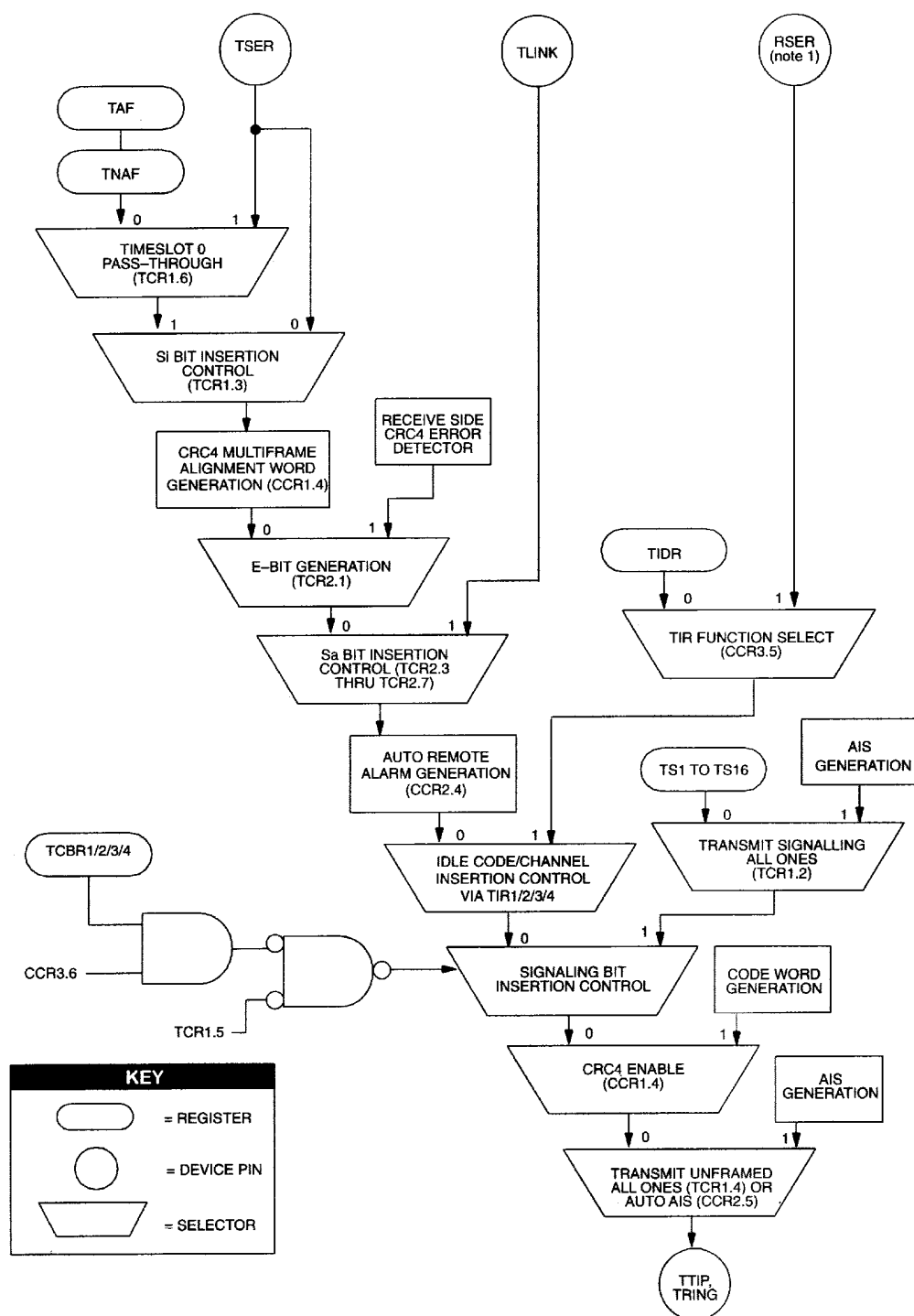
Figure 14-9. Transmit Data Flow
