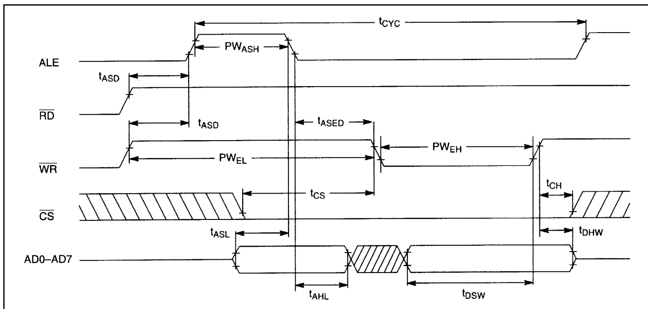
Figure 16-2. Intel Bus Write AC Timing
