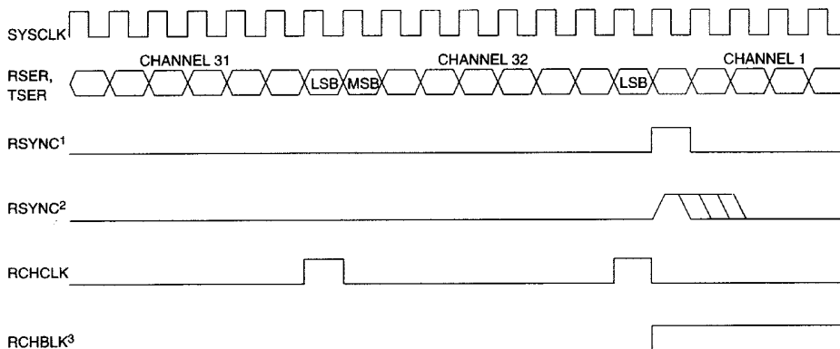
Figure 14-4. 2.048MHz Boundary Timing with Elastic Store(s) Enabled
