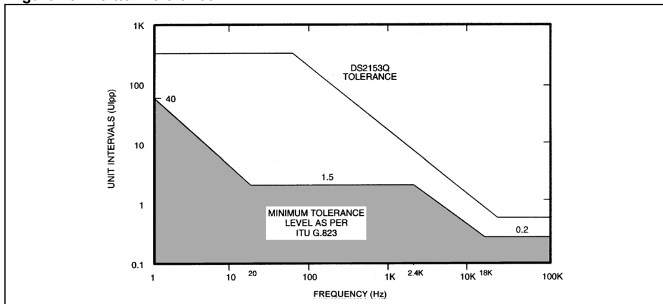
Figure 13-2. Jitter Tolerance
