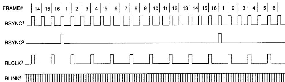
Figure 14-1. Receive Side Timing
