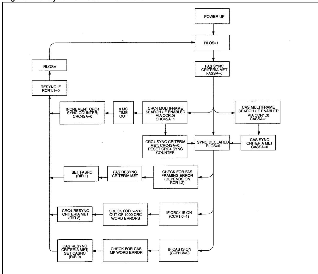
Figure 14-8. Synchronization Flowchart
