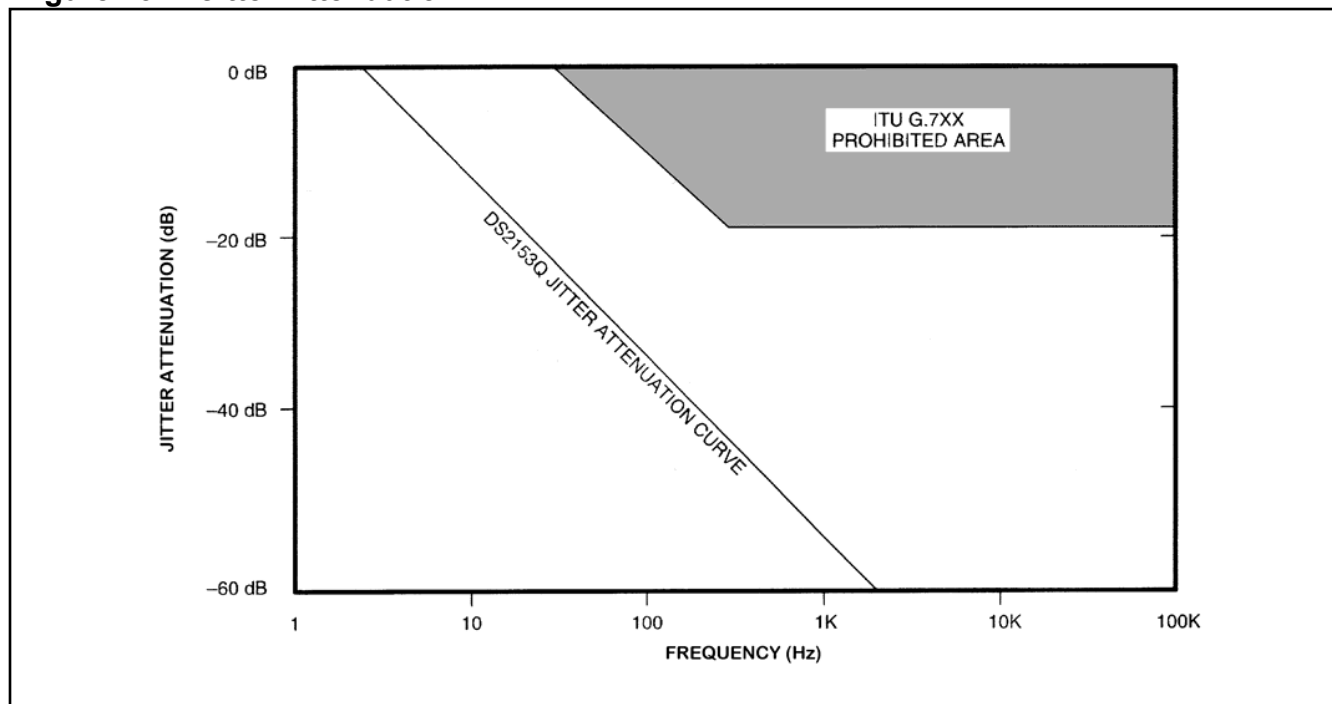
Figure 13-4. Jitter Attenuation
