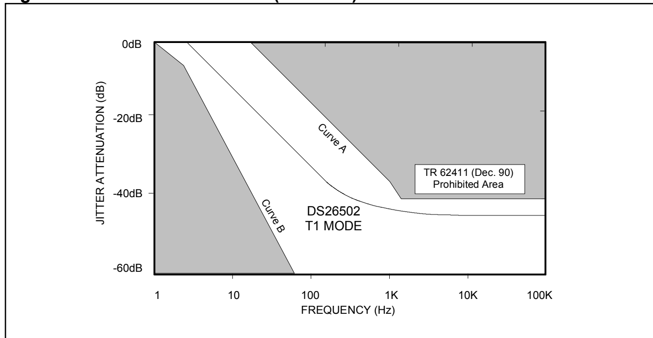
Figure 13-10. Jitter Attenuation (T1 Mode)
