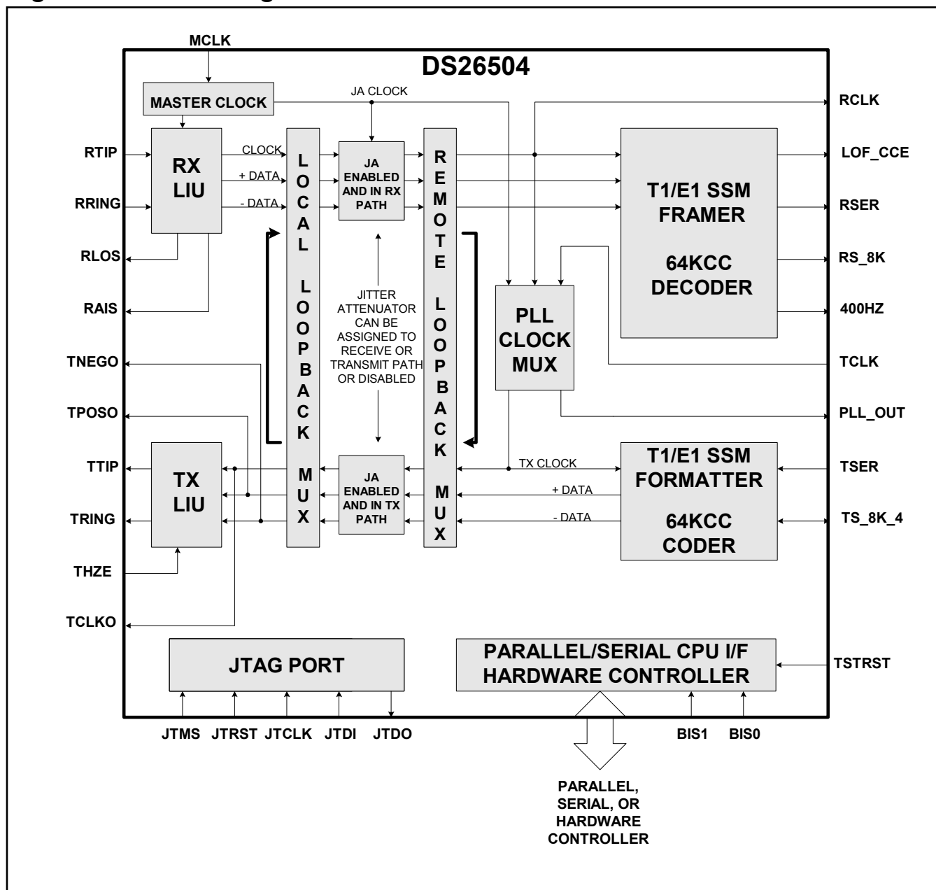
Figure 3-1. Block Diagram
