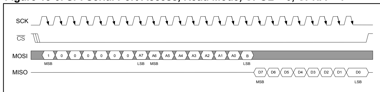
Figure 18-3. SPI Serial Port Access, Read Mode, CPOL = 0, CPHA = 1
