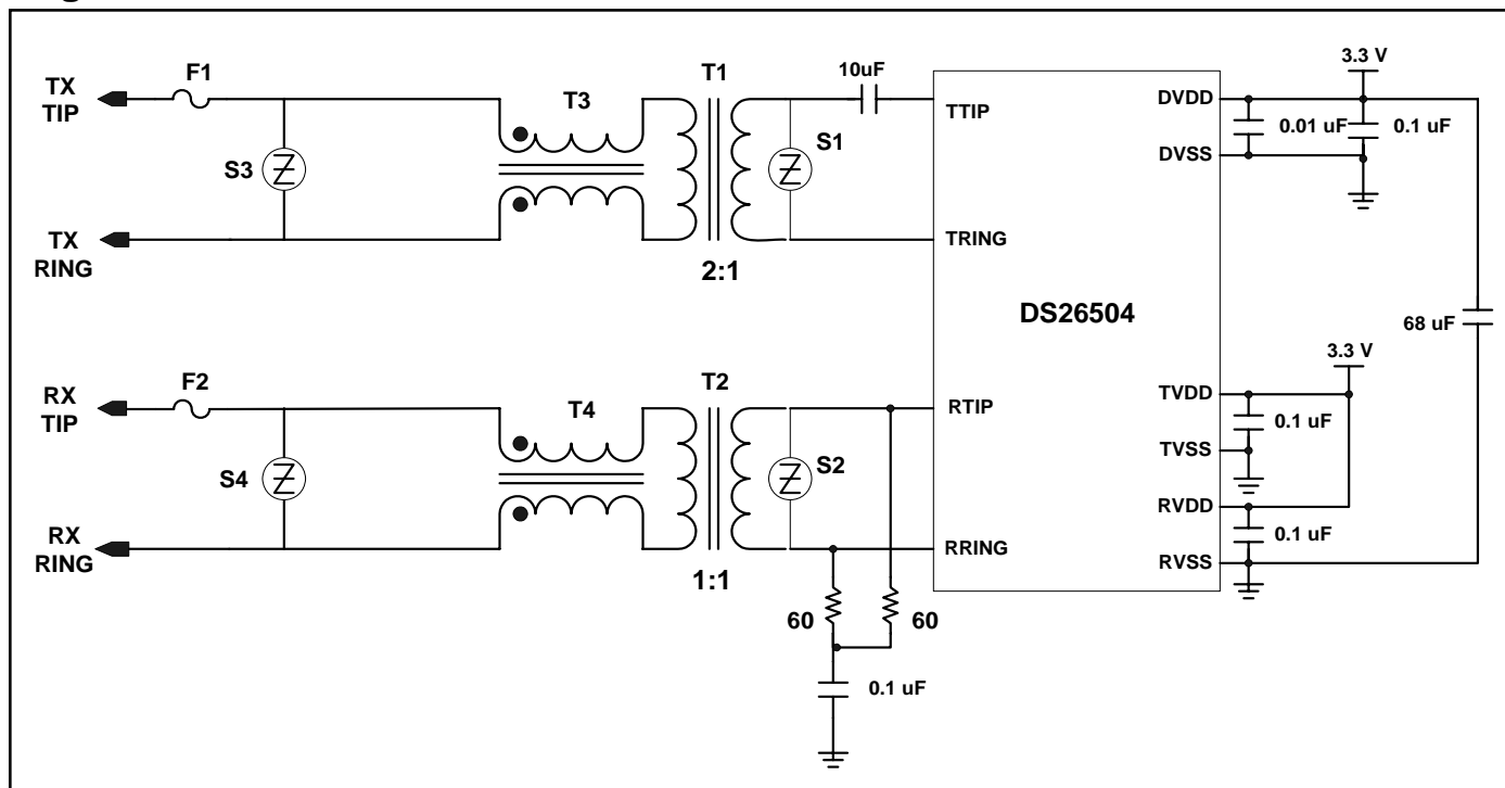
Figure 13-4. Software-Selected Termination, Metallic Protection
