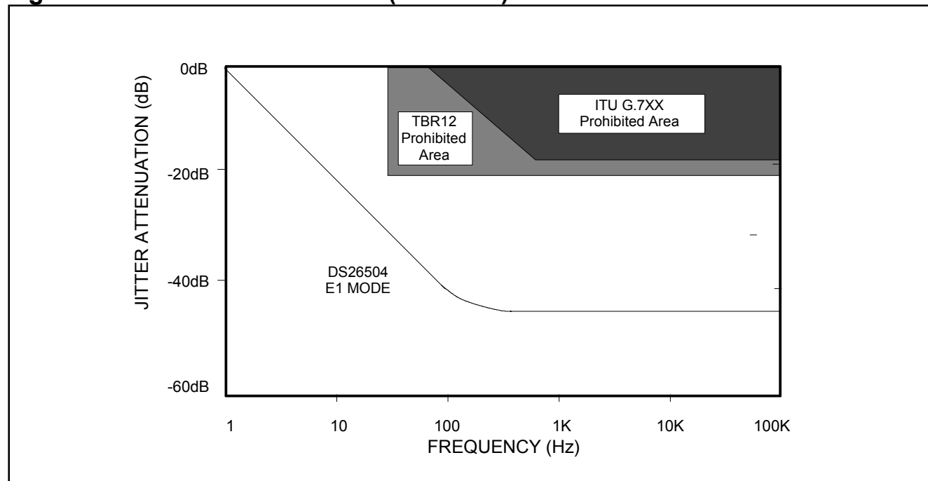
Figure 13-11. Jitter Attenuation (E1 Mode)
