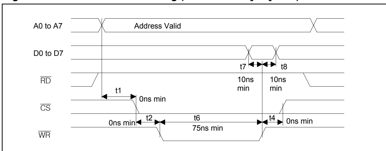
Figure 20-5. Intel Bus Write Timing (BTS = 0 / BIS[1:0] = 01)
