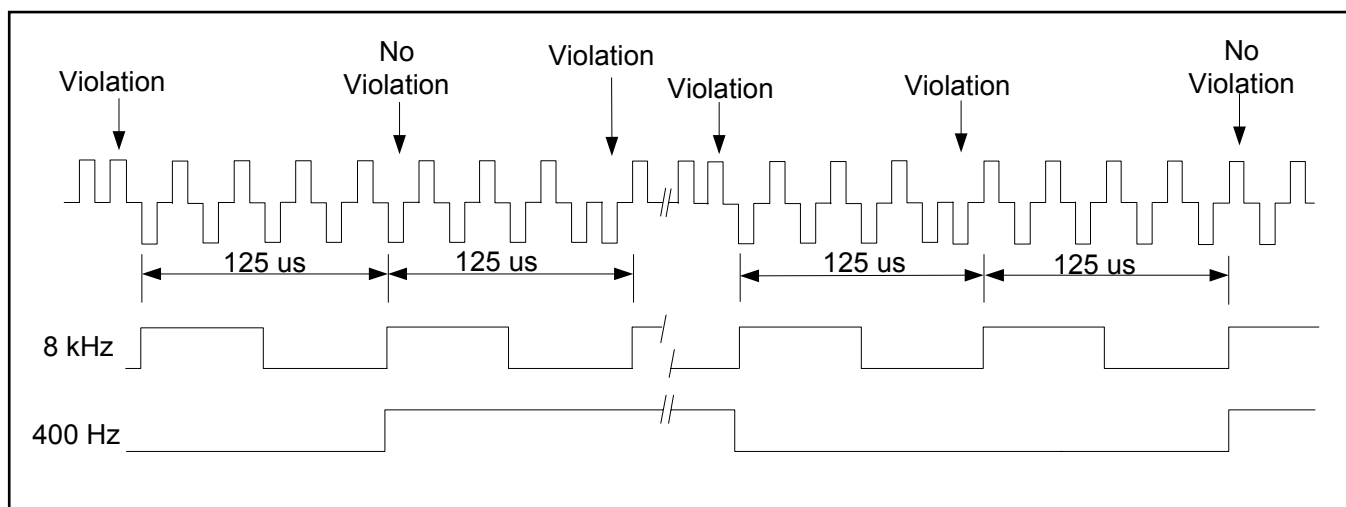
Figure 15-1. 64kHz Composite Clock Mode Signal Format
