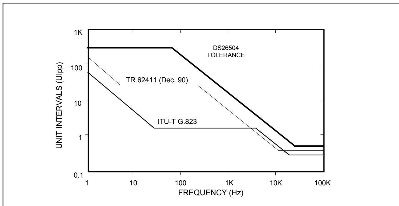
Figure 13-8. Jitter Tolerance (T1 Mode)
