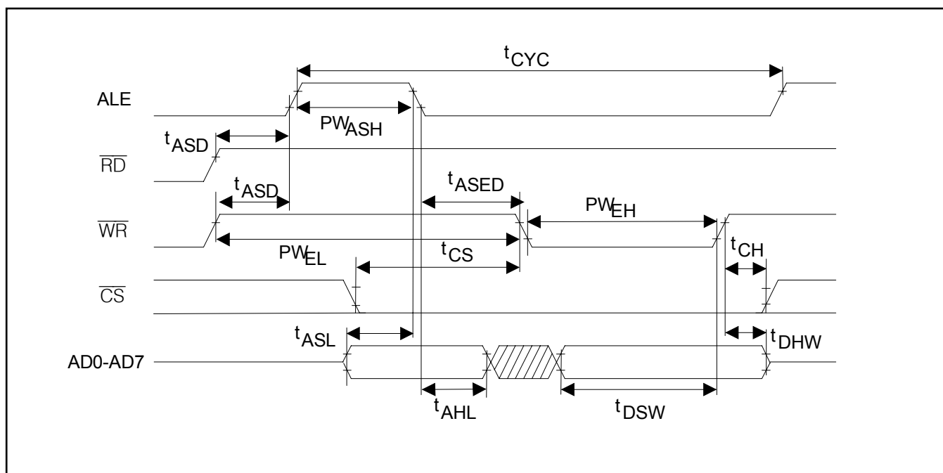
Figure 20-2. Intel Bus Write Timing (BTS = 0 / BIS[1:0] = 00)
