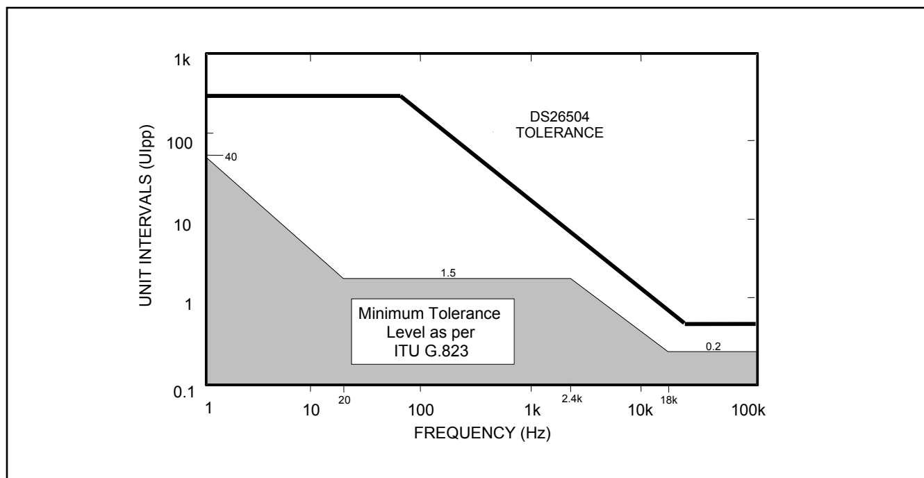
Figure 13-9. Jitter Tolerance (E1 Mode)
