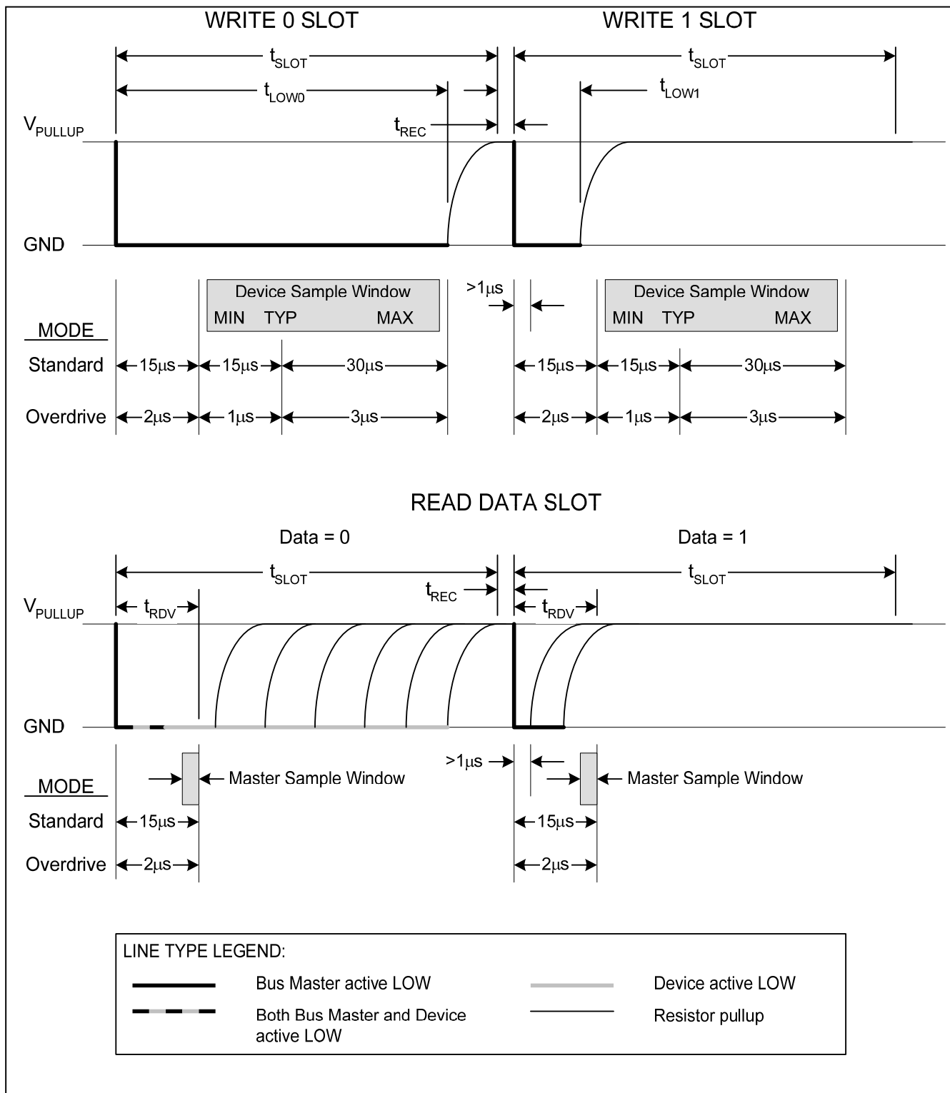
Figure 8. 1-Wire Write and Read Time Slots
