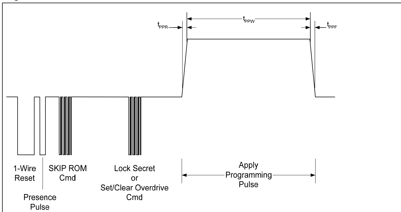
Figure 10. Lock Secret, Set/Clear Overdrive Function Commands
