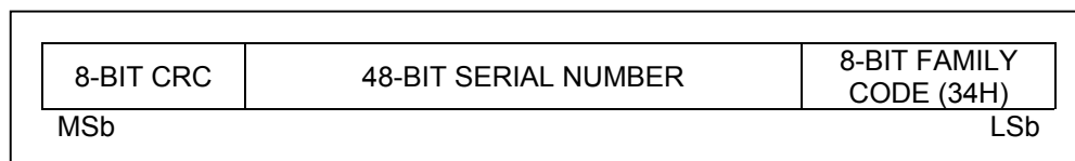
Figure 3. 1-Wire Net Address Format
