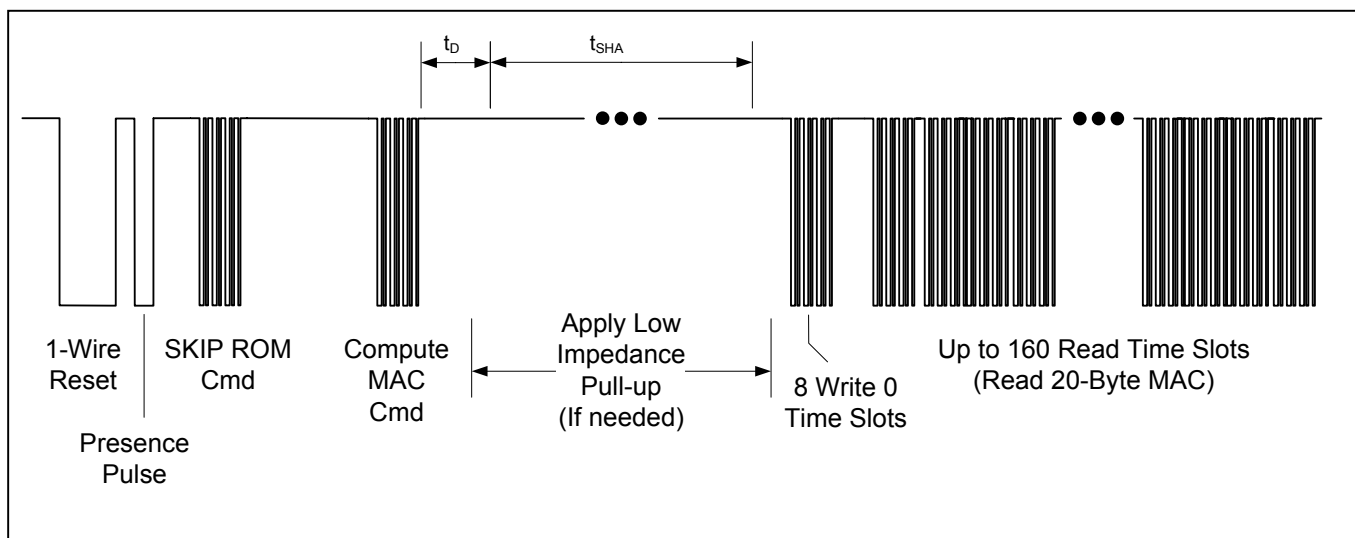
Figure 9. Compute MAC Function Command
