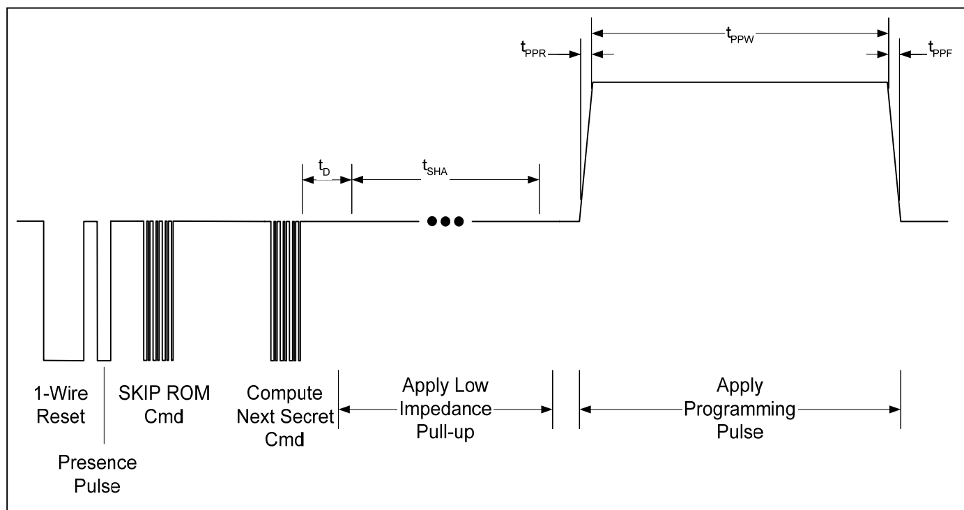
Figure 11. Compute Next Secret Function Command
