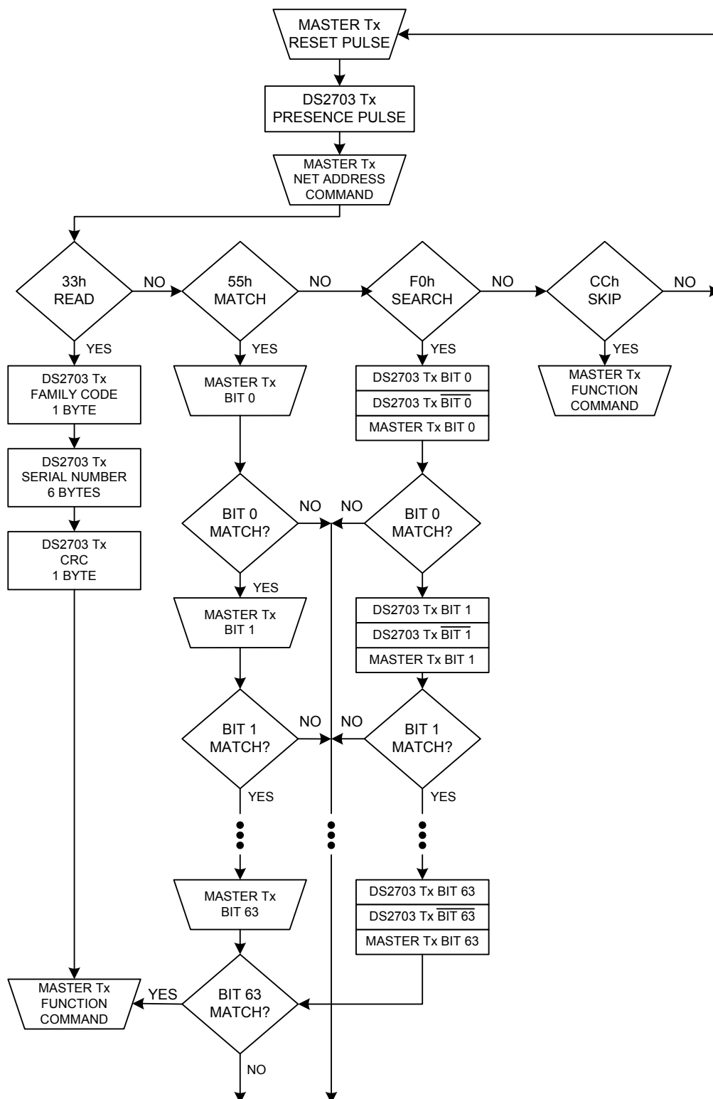
Figure 6. Net Address Command Flow Chart
