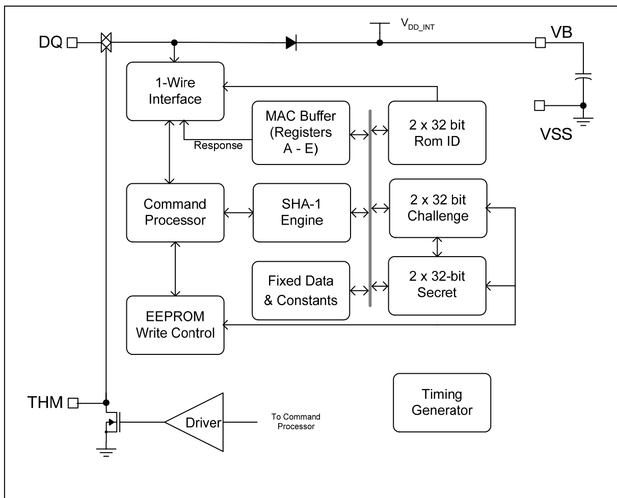
Figure 1. Block Diagram
