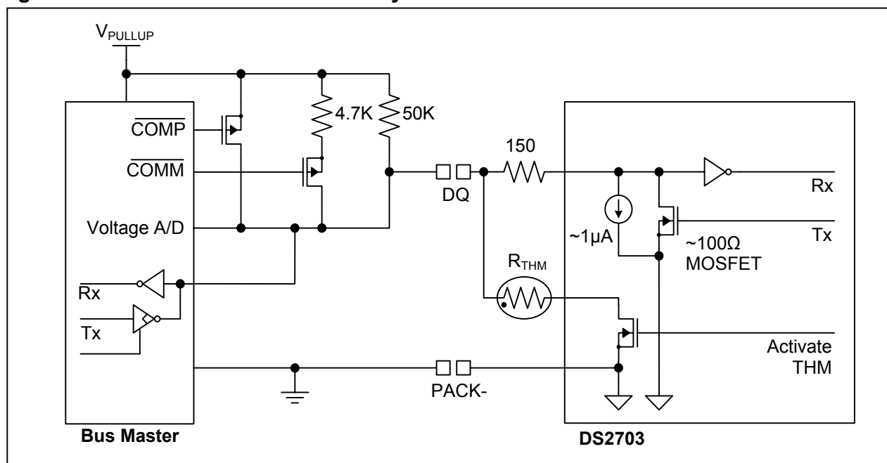
Figure 5. 1-Wire Bus Interface Circuitry
