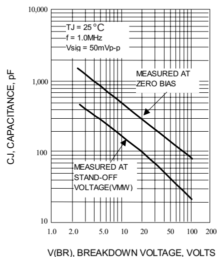
Fig. 4-TYPICAL JUNCTION CAPACITANCE
