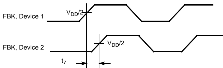
Figure 6. Device-Device Skew
