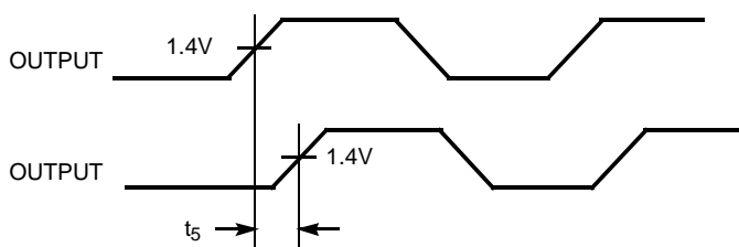
Figure 4. Output-Output Skew
