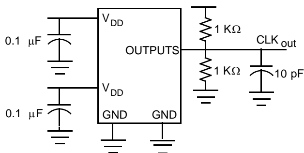
Test Circuit # 2
