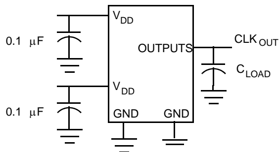
Figure 7. Test Circuit 1
