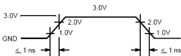
(c) TTL Input Test Waveform
