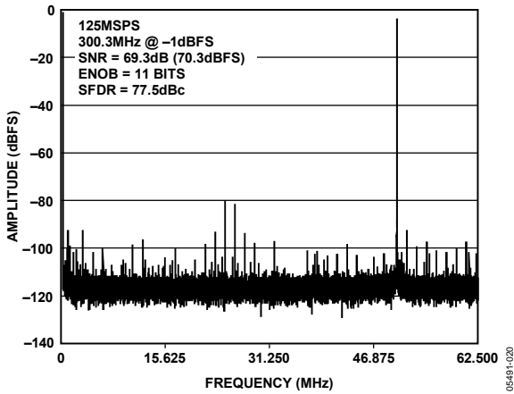
Figure 19. AD9246-125 Single-Tone FFT with f_{IN} = 300.3 MHz
