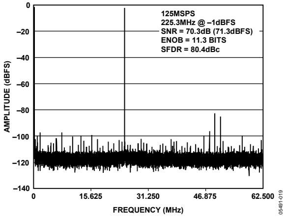
Figure 18. AD9246-125 Single-Tone FFT with f_{IN} = 225.3 MHz
