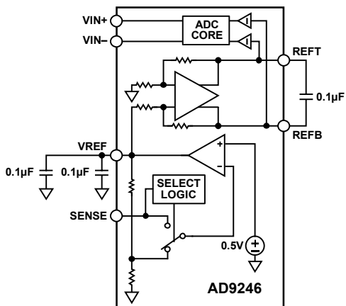
Figure 42. Internal Reference Configuration
