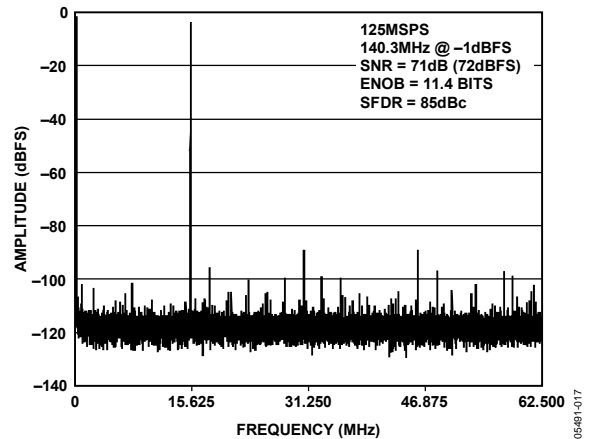
Figure 16. AD9246-125 Single-Tone FFT with f_{IN} = 140.3 MHz
