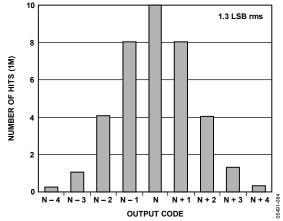
Figure 33. AD9246 Grounded Input Histogram
