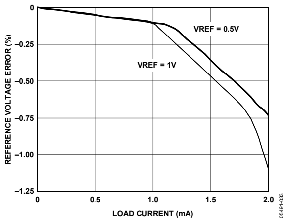
Figure 44. VREF Accuracy vs. Load
