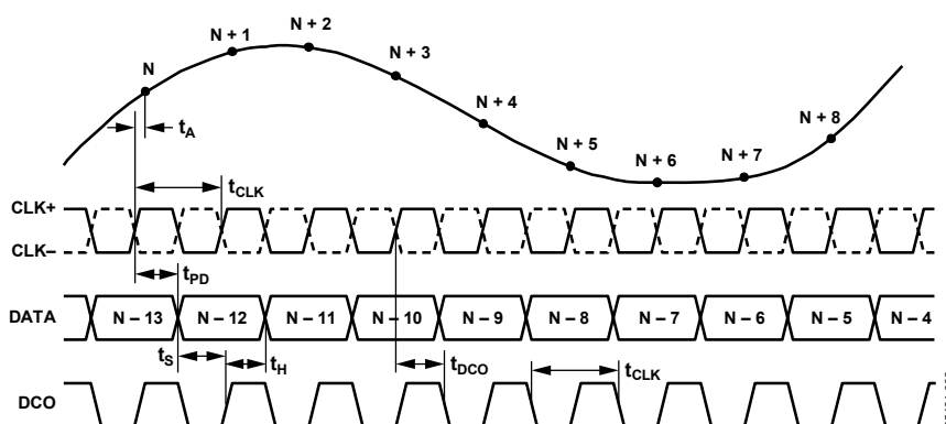
Figure 2. Timing Diagram
