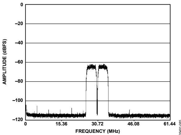
Figure 26. AD9246-125 Two 64k WCDMA Carriers with f_N = 215.04 MHz, f_s = 122.88 MSPS
