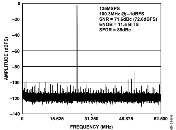
Figure 15. AD9246-125 Single-Tone FFT with f_{IN} = 100.3 MHz
