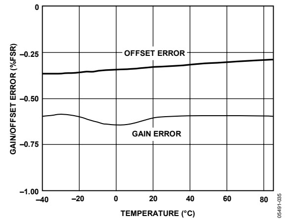
Figure 23. AD9246 Gain and Offset vs. Temperature
