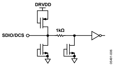
Figure 6. Equivalent SDIO/DCS Input Circuit
