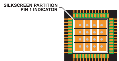
Figure 58. Typical PCB Layout
