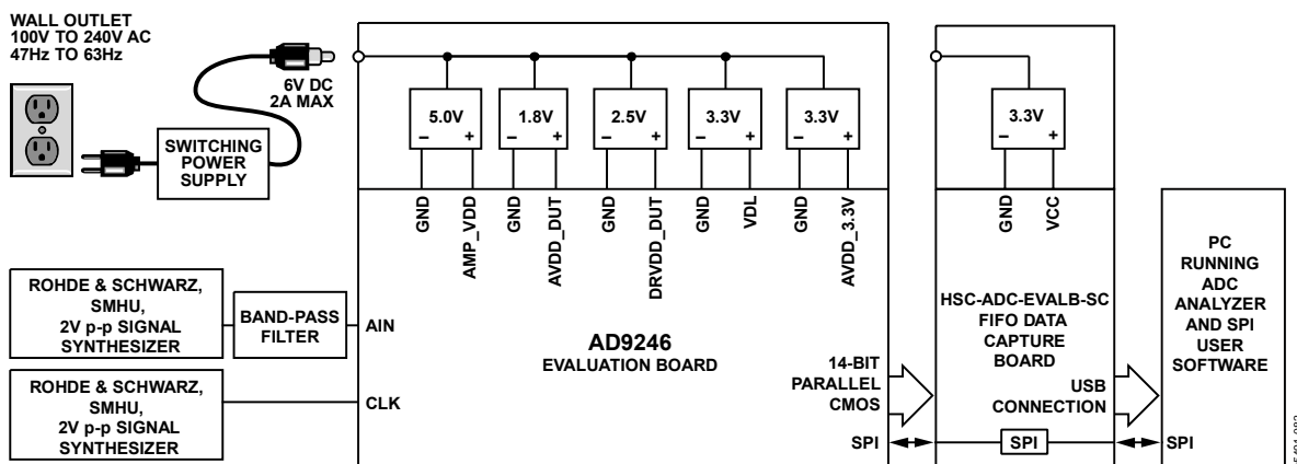
Figure 59. Evaluation Board Connection
