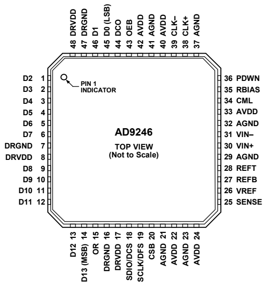
Figure 3. Pin Configuration
