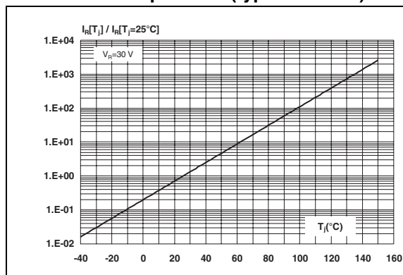
Figure 11. Relative variation of reverse leakage current versus junction temperature (typical values)
