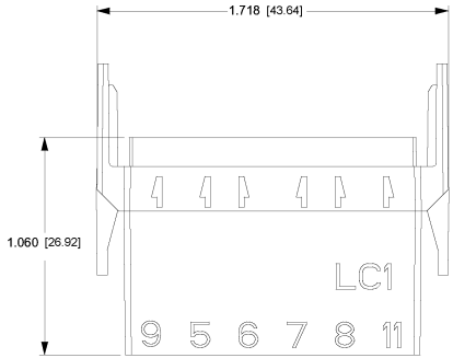
CONNECTOR HOUSING: FR-01
