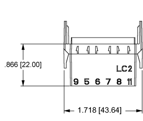
CONNECTOR HOUSING: FR-02
