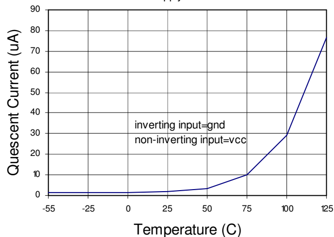
Quiescent current vs Temperature V_{supply} = 15V
