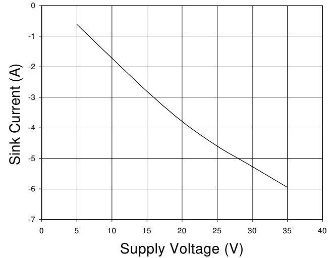
Output Sink Current vs. Supply Voltage
