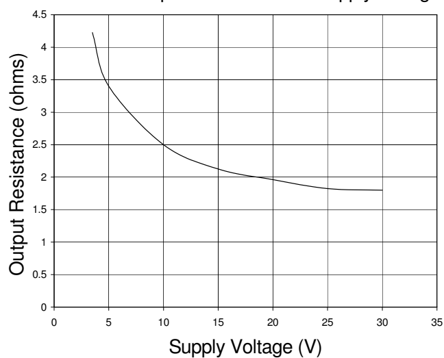
Fig. 30 Low State Output Resistance vs. Supply Voltage
