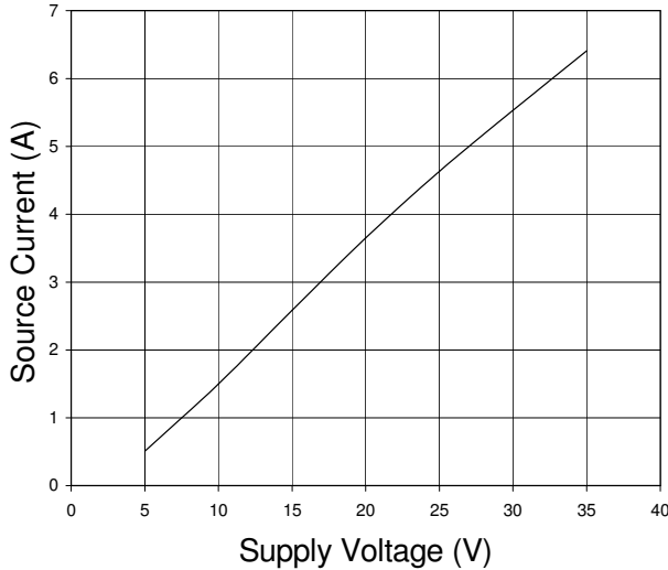
Output Source Current vs. Supply Voltage
