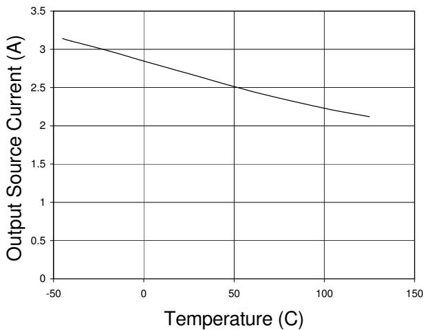
Output Source Current vs. Temperature V_{\text{SUPPLY}} = 15\text{V}
