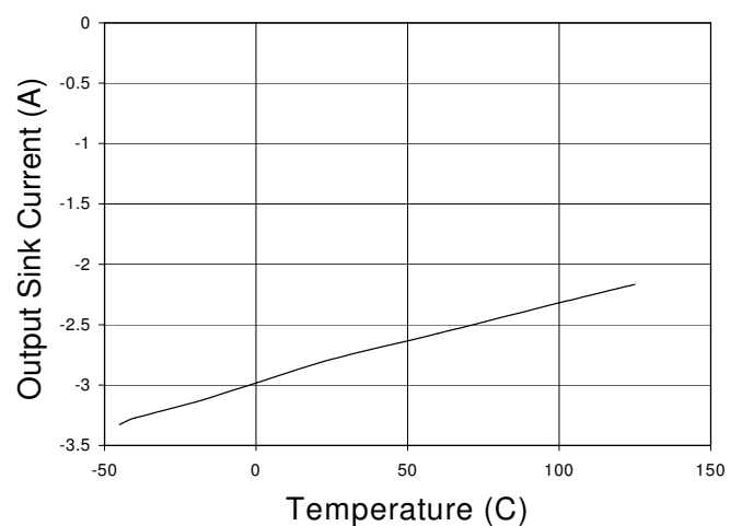
Output Sink Current vs. Temperature V_{\text{SUPPLY}} = 15\text{V}
