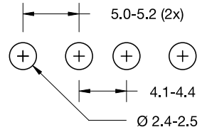
mounting pattern
