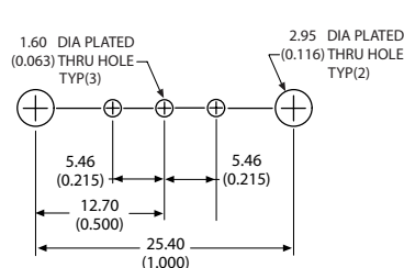
Recommended hole pattern for 8241-CL11G
