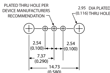
Recommended hole pattern for 8223-CL03G
