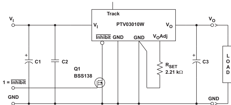
Figure 9. On/Off Inhibit Application Circuit
