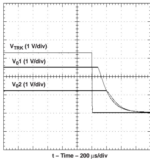
Figure 13. Simultaneous Power Down With Auto-Track Control
