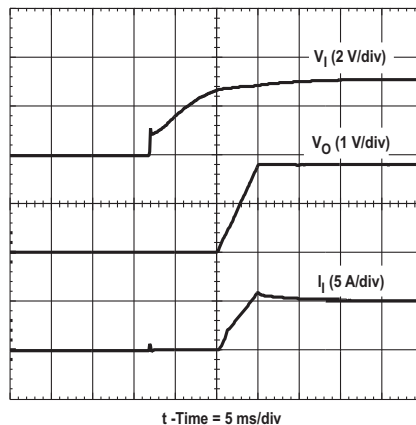
Figure 8. Power-Up Waveform
