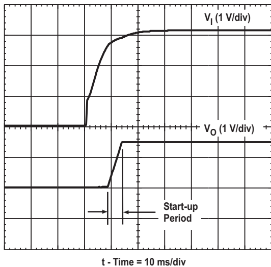
Figure 14. PTV03010W Start-Up
