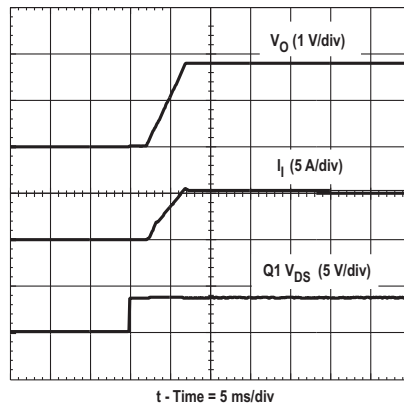
Figure 10. Inhibit Waveform
