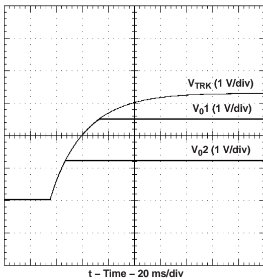
Figure 12. Simultaneous Power Up With Auto-Track Control
