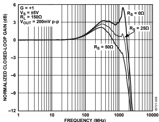
Figure 10. G = +1 Series Resistor ( R_S ) Optimization
