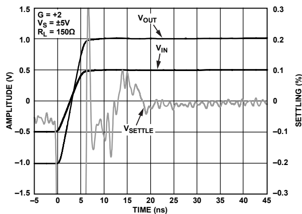
Figure 21. Short-Term 0.1% Settling Time
