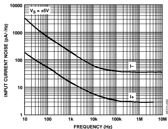
Figure 36. Input Current Noise vs. Frequency
