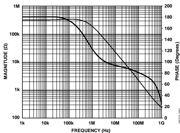
Figure 37. Transimpedance
