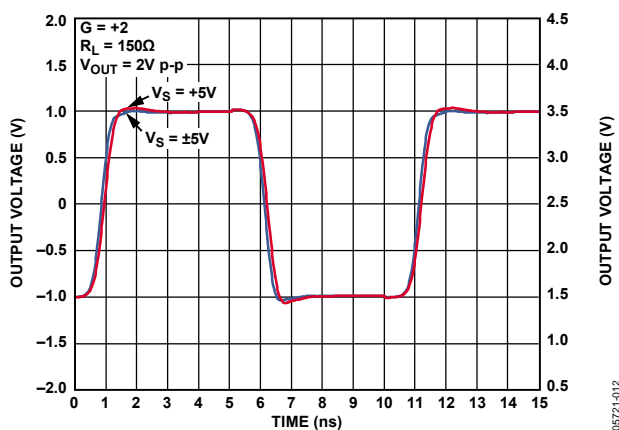
Figure 17. Large Signal Pulse Response for Various Supplies
