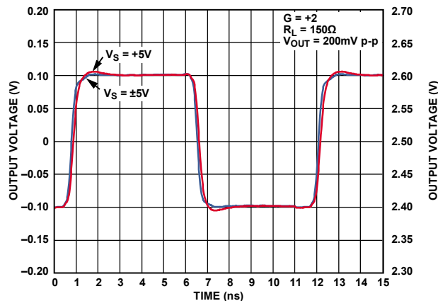
Figure 19. Small Signal Pulse Response for Various Supplies
