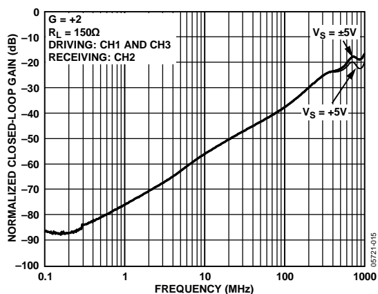
Figure 35. Worst-Case Crosstalk
