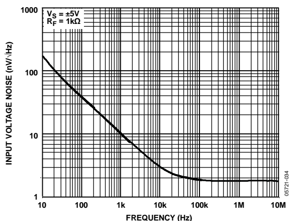
Figure 34. Input Voltage Noise vs. Frequency
