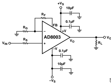
Figure 38. Noninverting Gain
