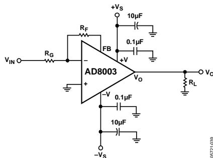
Figure 39. Inverting Gain
