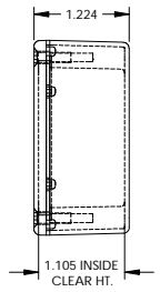
DETAIL D SCALE 6 : 1
