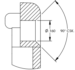
DETAIL D SCALE 6:1
