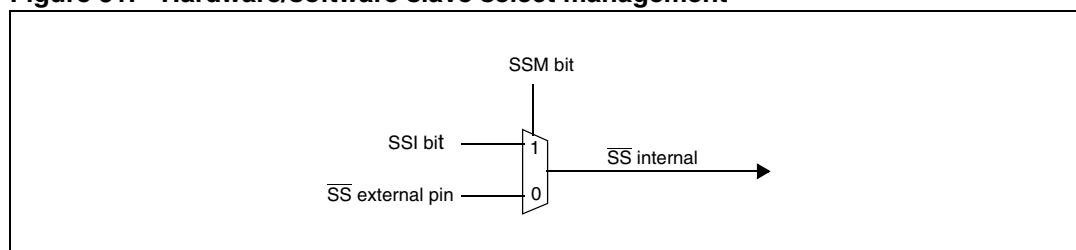
Figure 51. Hardware/software slave select management
