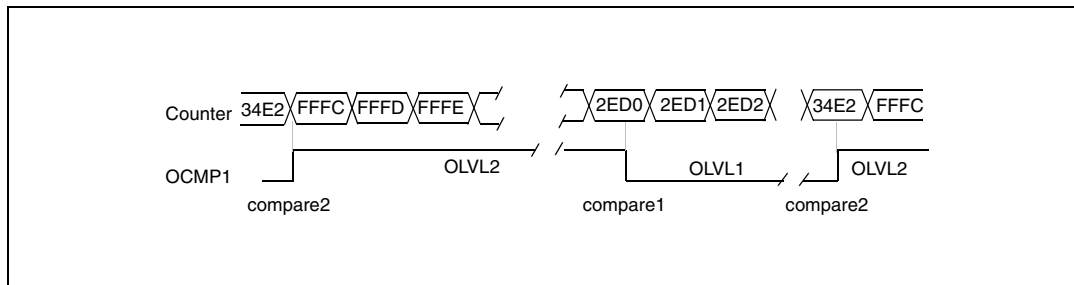
Figure 46. Pulse width modulation mode timing example with two output compare functions (1)(2)
