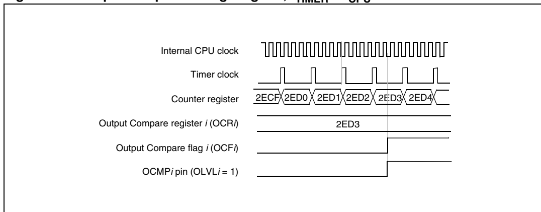
Figure 43. Output compare timing diagram, f_{\text{TIMER}} = f_{\text{CPU}}/4
