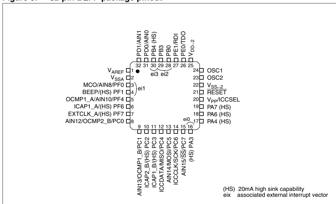
Figure 3. 32-pin LQFP package pinout
