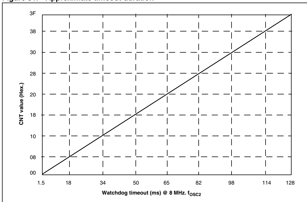
Figure 31. Approximate timeout duration
