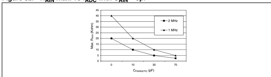
Figure 82. R_{AIN} max. vs f_{ADC} with C_{AIN} = 0\text{pF}^{(1)}
