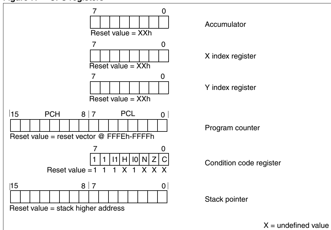
Figure 7. CPU registers
