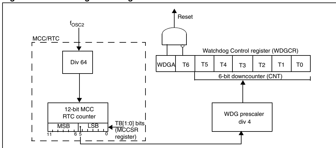
Figure 30. Watchdog block diagram
