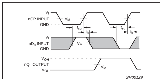
Waveform 3. Set up and hold times.
