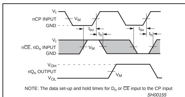
Waveform 3. Data Setup and Hold Times for the D_n or CE input to the CP input
