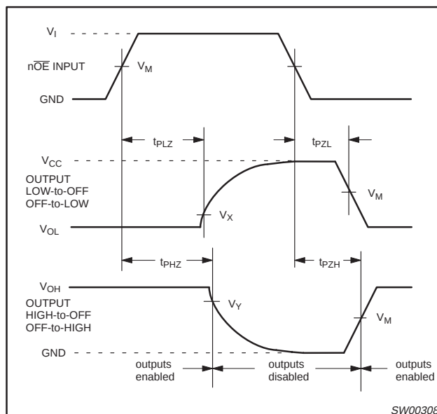
Waveform 4. 3-State Enable and Disable Times
