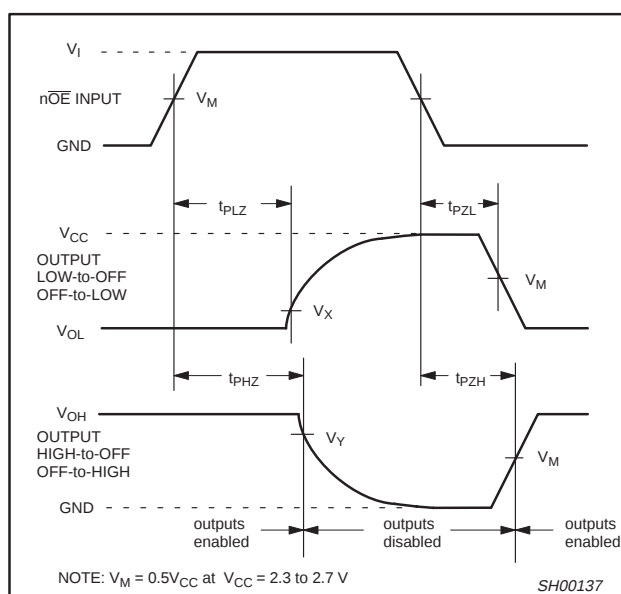
Waveform 6. 3-State enable and disable times
