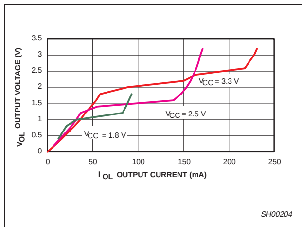
Figure 2. Output voltage ( V_{OL} ) vs. output current ( I_{OL} )
