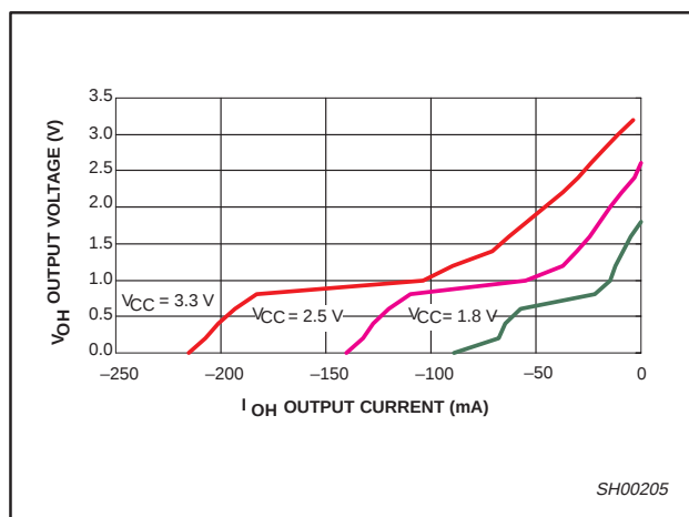
Figure 3. Output voltage ( V_{OH} ) vs. output current ( I_{OH} )
