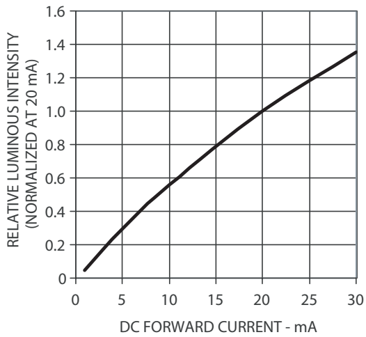
Figure 7. Relative Intensity vs Forward Current
