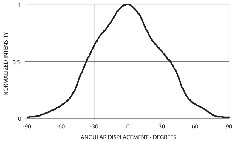
Figure 10. Radiation pattern-Major Axis
